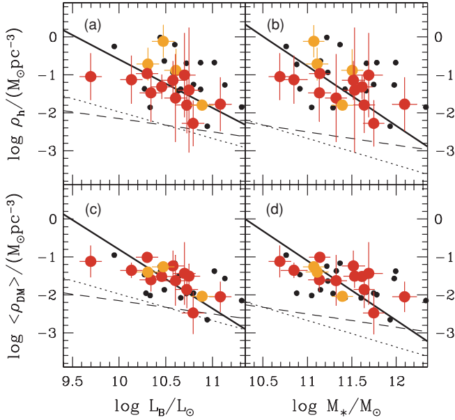
Figure 4. Central halo density \rho_h and average dark matter density ( \rho_{DM} ) inside 2r_{\text{eff}} vs. luminosity L_B (a, c) and stellar mass M_* (b, d). Solid lines: fits including all Coma galaxies; dotted and dashed lines: spiral galaxy scaling relations as in Figure 1.
