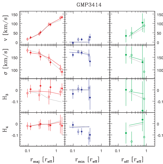
Figure 10. Upper panel: joint ground based and HST photometry of GMP 3414/NGC 4871. Lines: best-fit deprojection. Lower panel: stellar kinematics along major axis (left/red), along the minor axis (middle/blue), and along a third axis parallel to the major axis with an offset of r_{\text{eff}}/2 (right/green); filled and open circles refer to different sides of the slits; dotted: best-fit model without dark matter.
