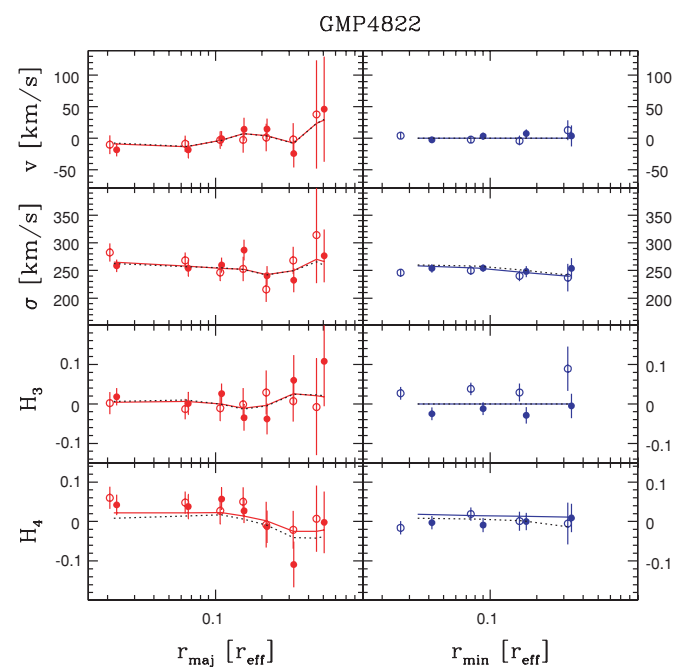
Figure 11. Same as Figure 10 but for GMP 4822/NGC 4841A.
