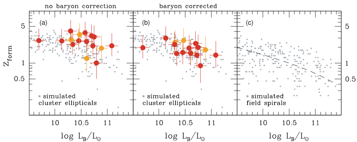
Figure 8. Comparison between assembly redshifts z_{\text{form}} of simulated and observed galaxies (symbols as in Figure 7). Both formation redshift estimates for Coma galaxies with and without baryon correction are shown (panels a and b). For comparison, panel (c) shows formation redshifts of simulated spirals (dots) and of observed spirals (dashed line; see Equation (12)). Simulated galaxies from the semi-analytic models of De Lucia & Blaizot (2007).
