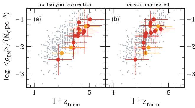
Figure 9. Average halo density ( \langle \rho_{DM} \rangle ) vs. assembly redshift. Large symbols: Coma galaxies without baryon correction (a) and with baryon correction (b). Small symbols: simulated cluster ellipticals and simulated field spirals from the semi-analytic models of De Lucia & Blaizot (2007).
