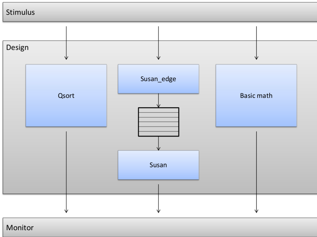
Figure 4.3: MiBench design
