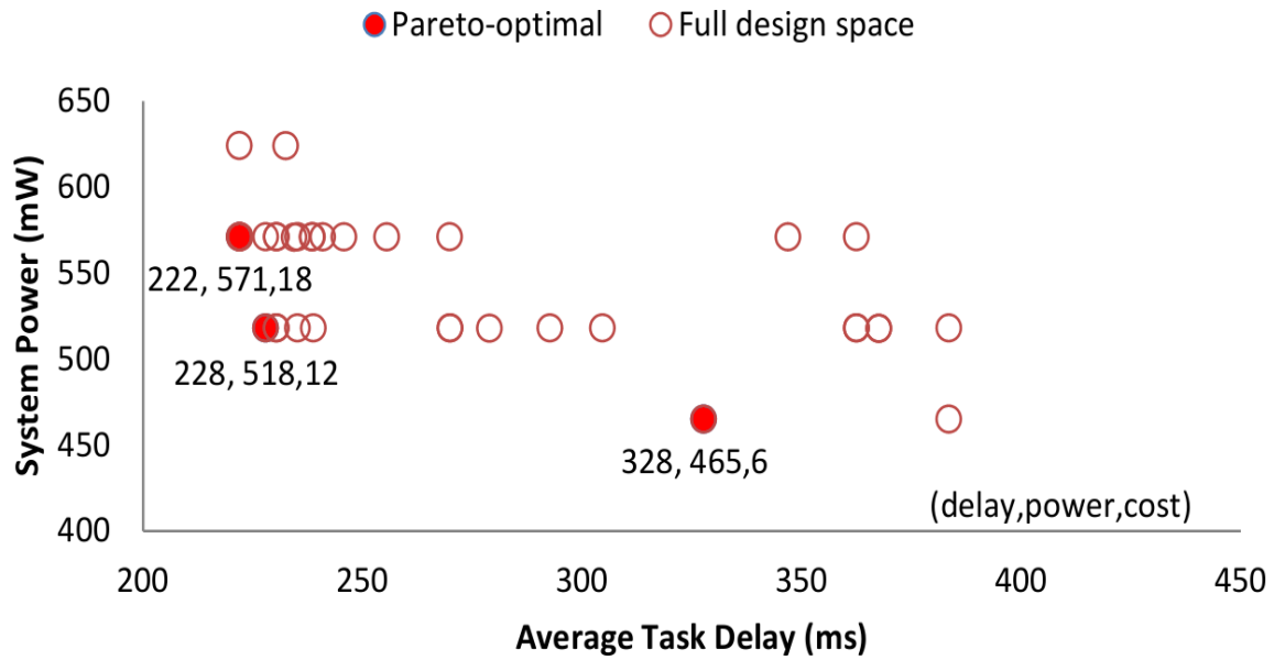
Figure 4.4: Pareto-optimal front for MiBench DSE
