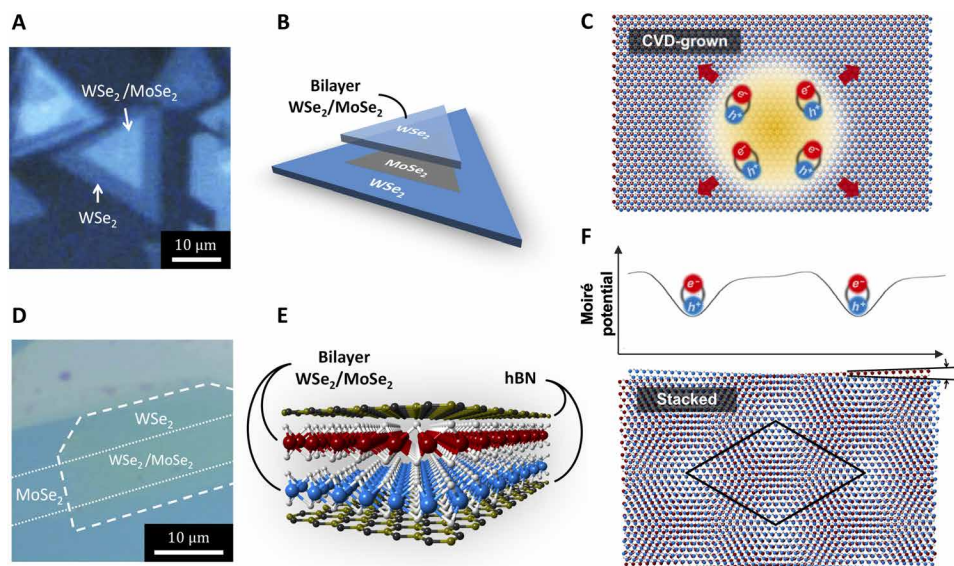
Fig. 1. Two types of WSe 2 /MoSe 2 heterostructures and the absence/presence of moiré superlattice. (A) Optical images of CVD-grown sample A-1. (B) Illustrated CVD-grown hBL, which consists of a monolayer WSe 2 covering on top of a monolayer MoSe 2 -WSe 2 lateral heterostructure. (C) Schematics of exciton diffusion in a CVD-grown WSe 2 /MoSe 2 bilayer with a commensurate structure. (D) Optical image of mechanically stacked WSe 2 /MoSe 2 hBL sample B-1. (E) Illustration of the hBN-encapsulated WSe 2 /MoSe 2 hBL. (F) Impeded exciton diffusion by the moiré potential in a MET hBL. The moiré supercell size decreases with an increasing twist angle \theta between the two layers.
