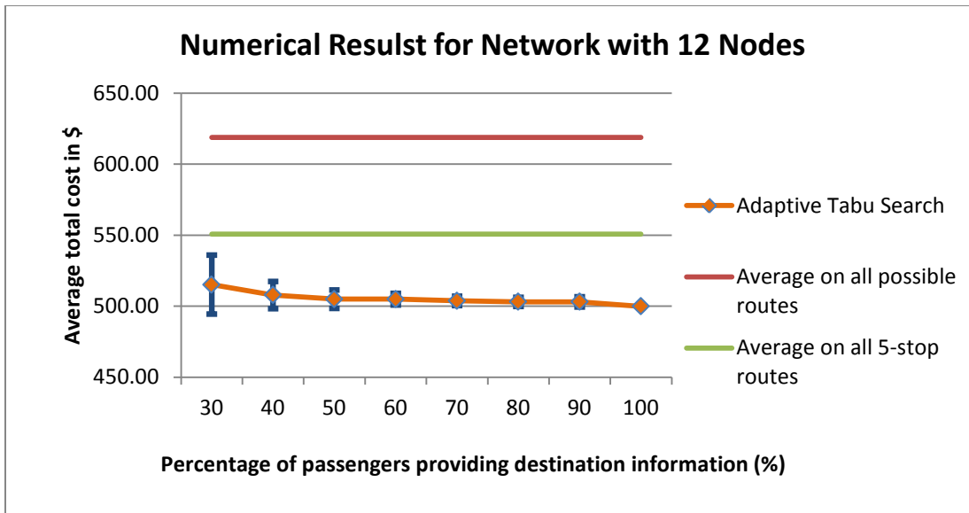
Figure 6.1: Numerical Results for 12-node Network
