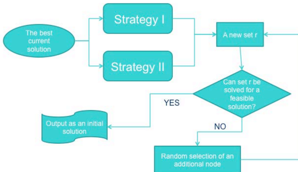
Figure 3: Initial Solution Construction.
