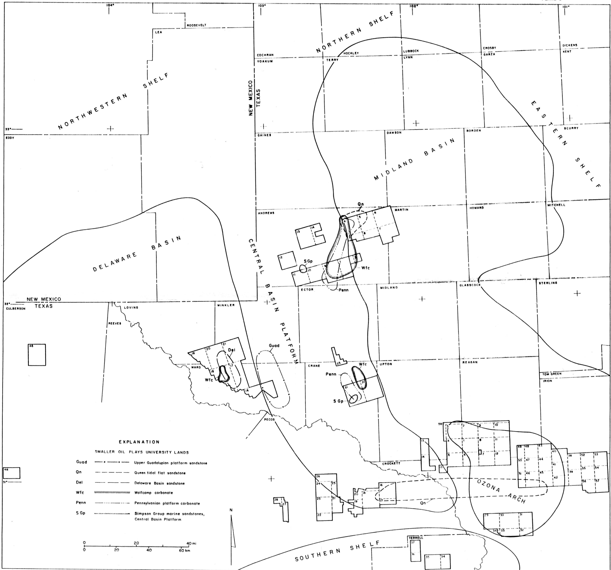
Plate 3. Location of minor University Lands oil-producing plays.
