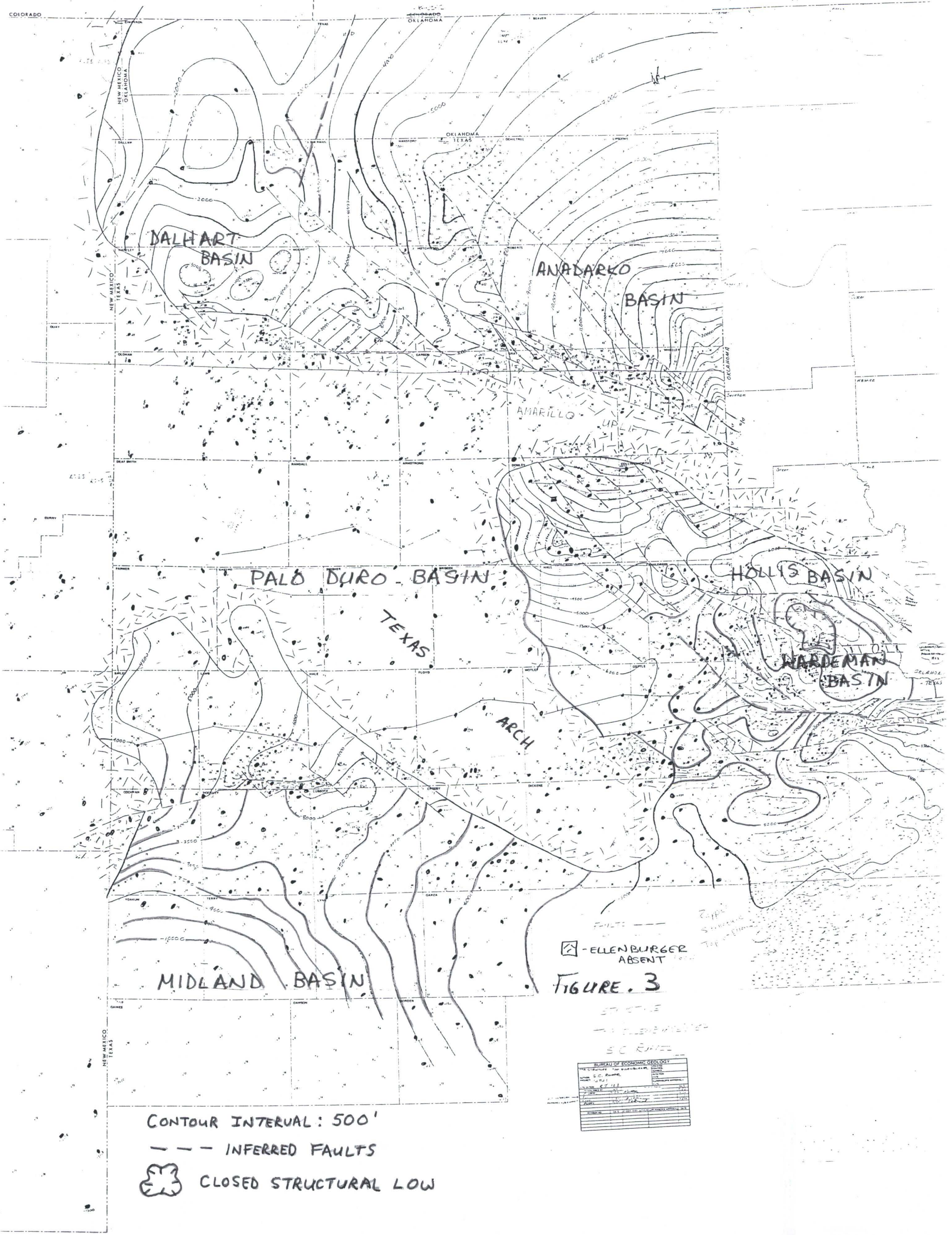
Figure 3. Structure on top of the Ellenburger Group (Lower Ordovician) in the Texas Panhandle area. Faults are interpretive based, for the most part, on well control only.
