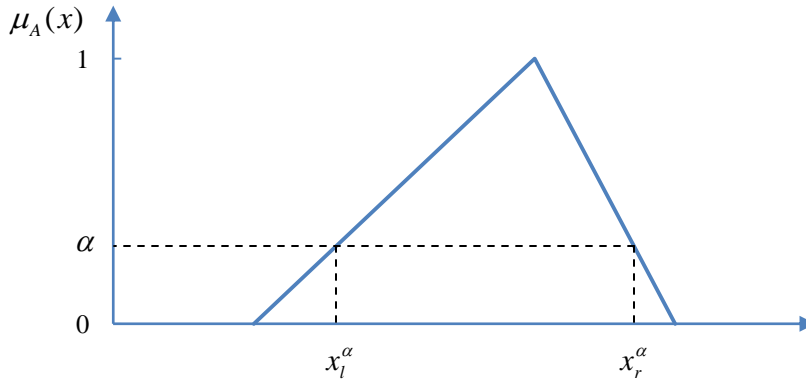
Figure 3: \alpha -cut on Triangular Membership Function
