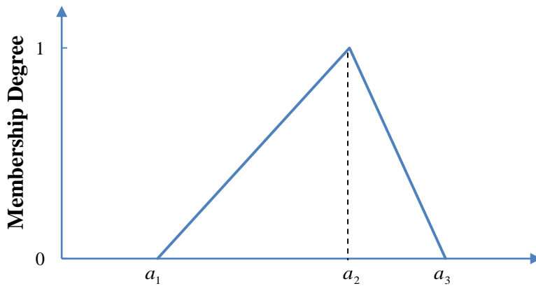
Figure 2: Triangular Fuzzy Number Function
