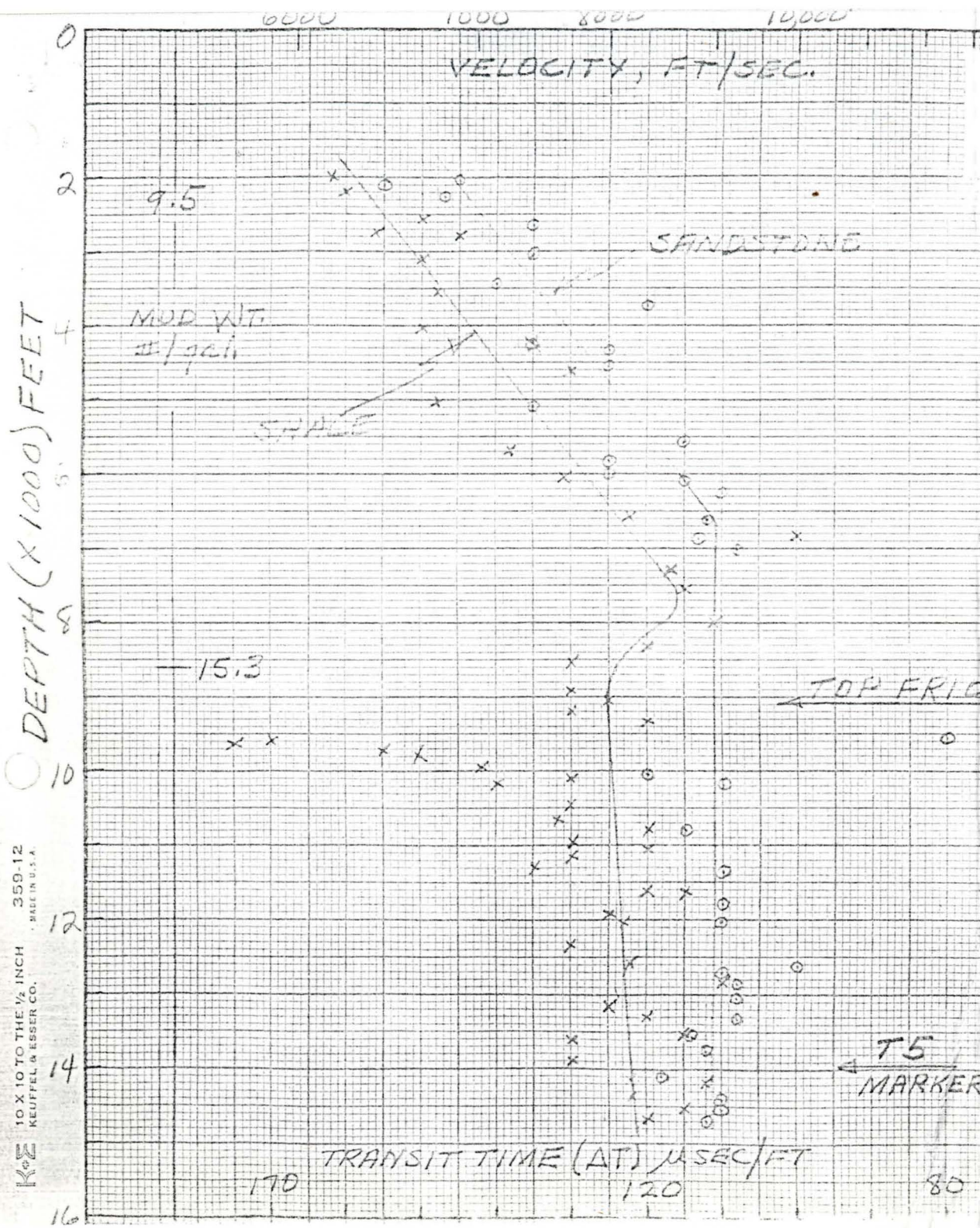
Figure 13. Shale and sandstone velocity, shale resistivity, and log-interpreted salinity from the Department of Energy and General Crude Oil No. 1 Pleasant Bayou geothermal test well, Austin Bayou Prospect, Brazoria County.
