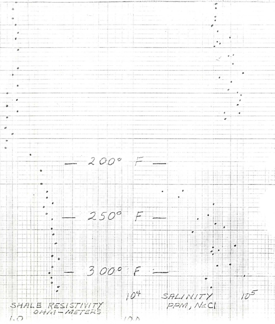
Figure 13. Shale and sandstone velocity, shale resistivity, and log-interpreted salinity from the Department of Energy and General Crude Oil No. 1 Pleasant Bayou geothermal test well, Austin Bayou Prospect, Brazoria County.
