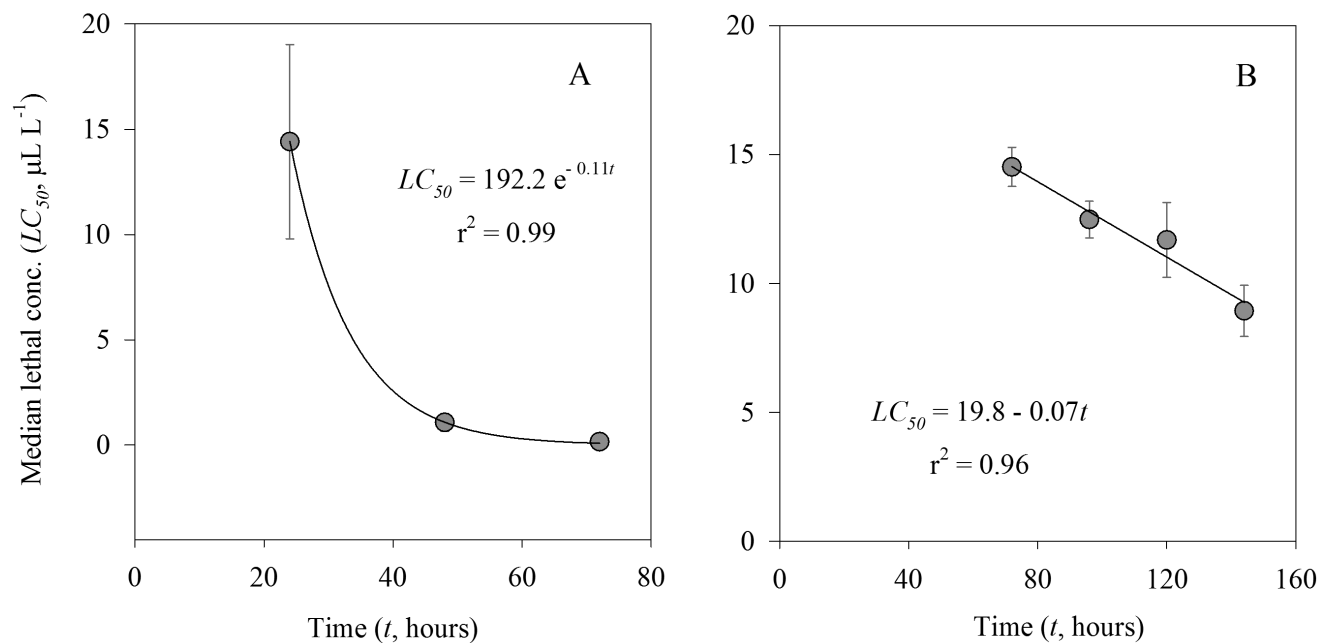
Figure 4. Relationships between median lethal concentration ( LC_{50} , \mu\text{L L}^{-1} ) and incubation time ( t , hours) of ephyra larvae of the scyphozoan Aurelia aurita (A) and cydippid larvae of the ctenophore Mnemiopsis leidyi (B) exposed to crude oil. doi:10.1371/journal.pone.0074476.g004
