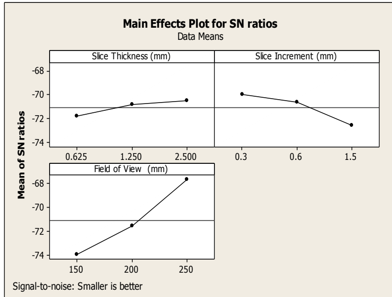
Fig. 3: Effect of CT image construction parameters on volumetric error
