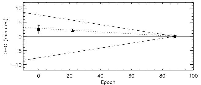
Fig. 3. Observed transit time deviations from our ephemeris. The data are from Gillon et al. (2007b, square), an average of the G07, D07, and S08 values (triangle), and this paper (star). For the later two values the error bars are smaller than the size of the points. The dashed lines give the \pm 1\sigma range allowed by the uncertainty in the orbital period propagated backwards in time. The dotted line shows the trend expected due to the revised value of the period based on fitting the transit times.
