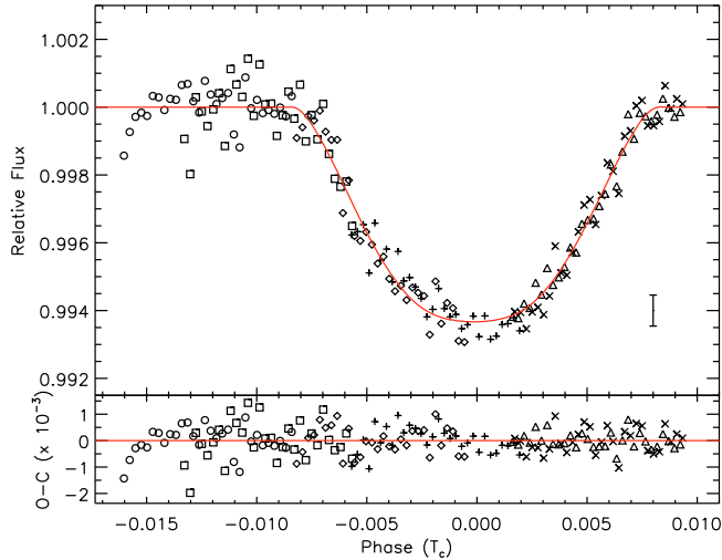
Fig. 1. Top: observed transit light curve for GJ 436b (points) with best fit from our analysis (line) phased to the central transit time. The bar on the right indicates the average error size. Bottom: residuals from the fit (points), which have a rms of 5.2 \times 10^{-4} . The different point styles in both panels indicate data from the different visits.
