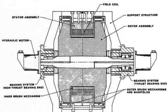
Fig. 1. Section through compact homopolar generator
