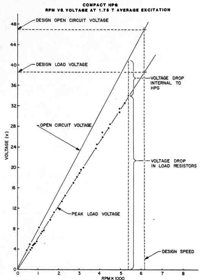
Fig. 3. HPG output voltage vs rotor speed
