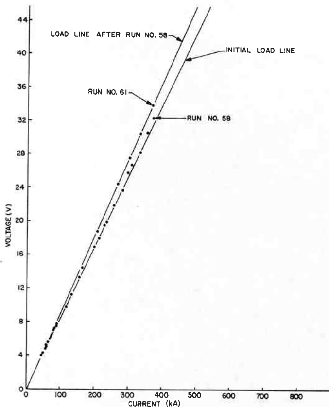
Fig. 4. Peak load voltage vs discharge current.
