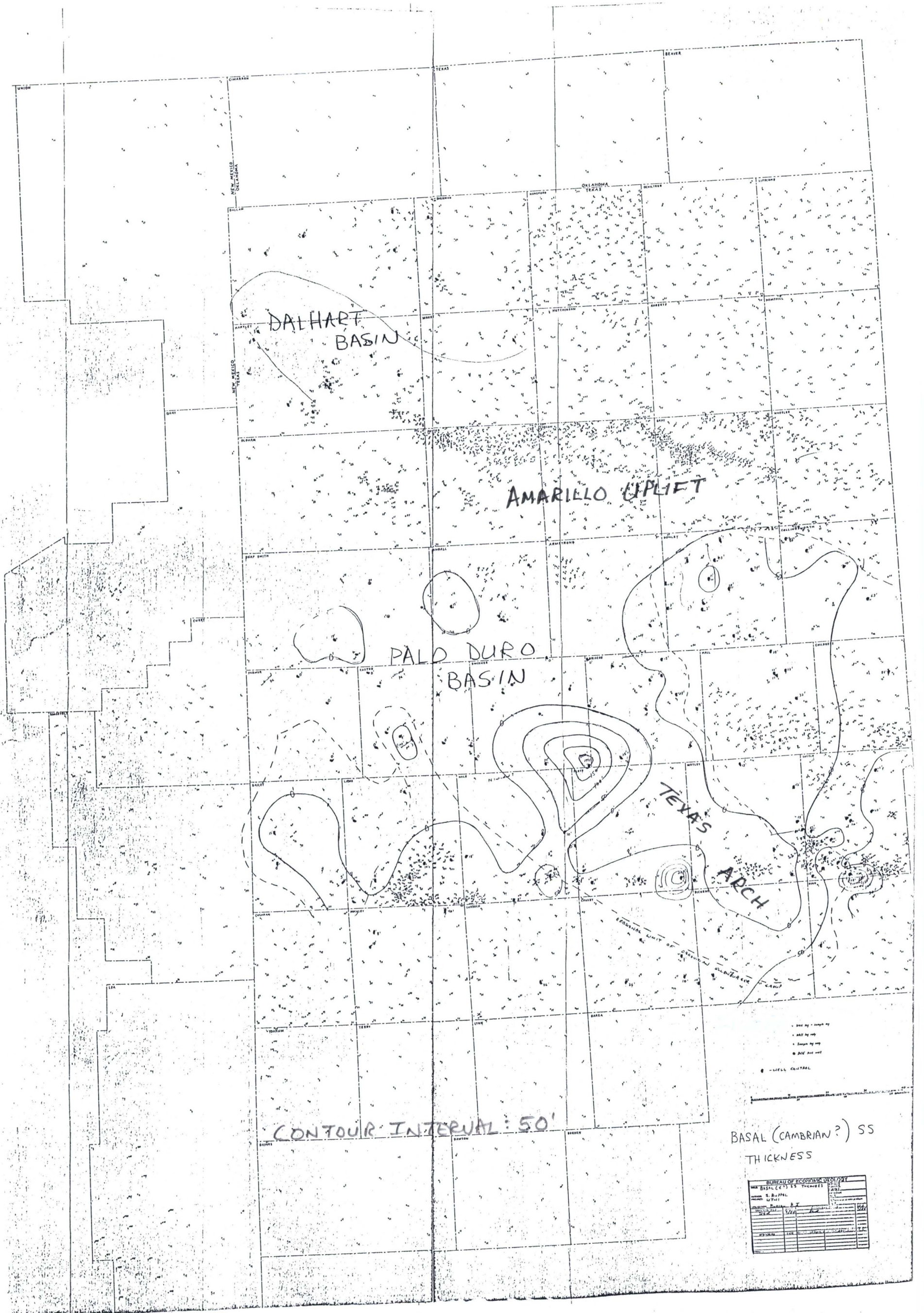
Figure 6. Thickness of Cambrian (?) basal clastic deposits in the Texas Panhandle area.
