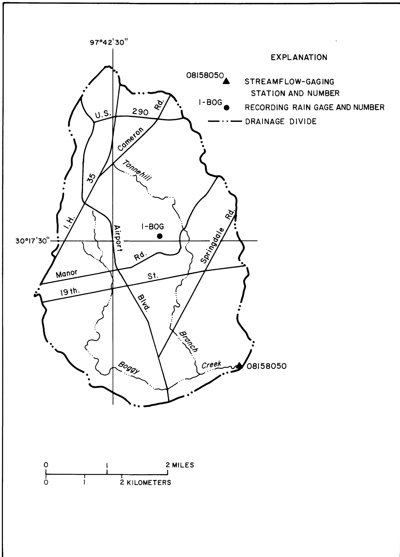
Figure 4.—Boggy Creek study area showing location of streamflow stations and recording rain gages.
