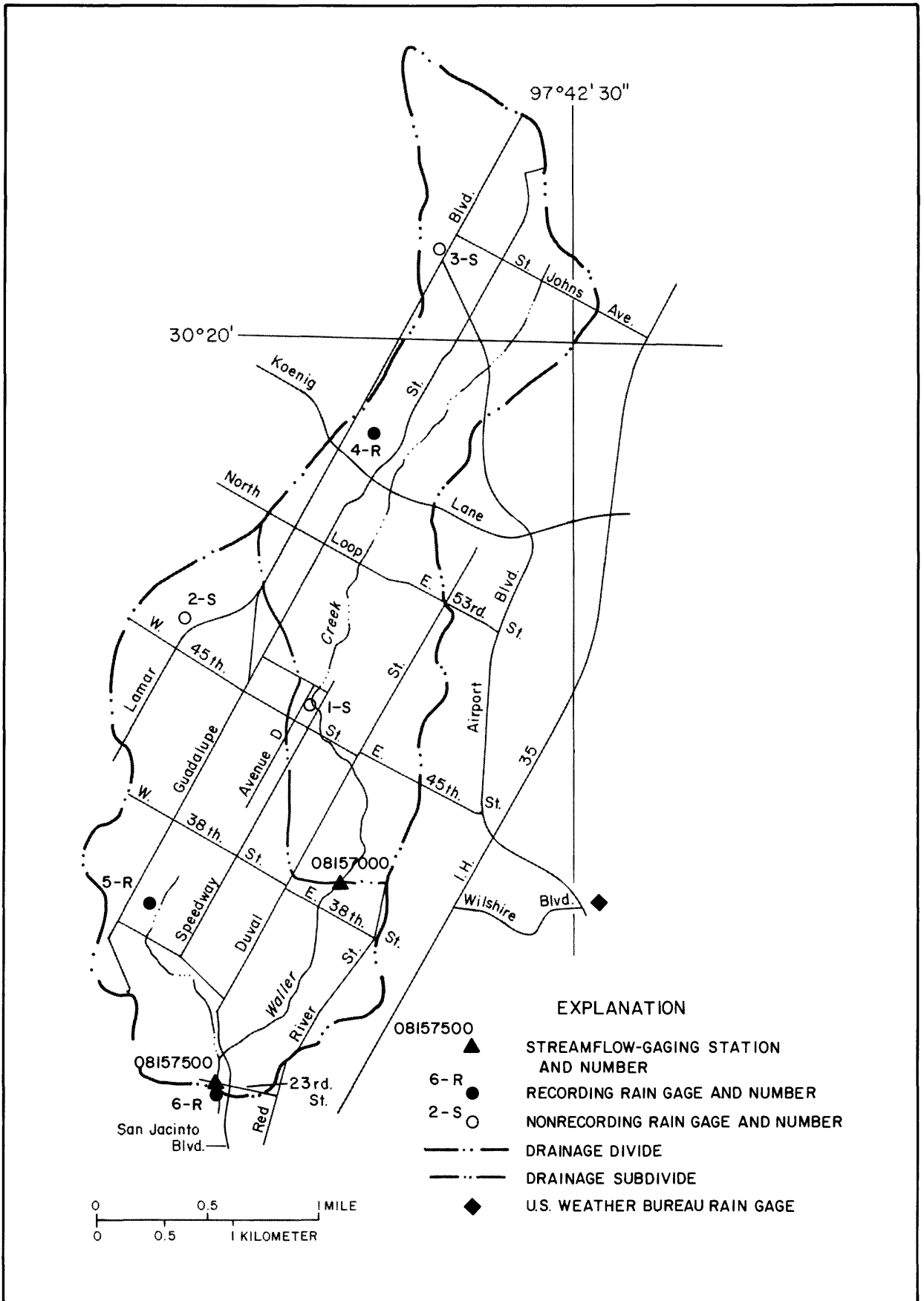
Figure 3.--Waller Creek study area showing location of streamflow stations and recording and nonrecording rain gages.
