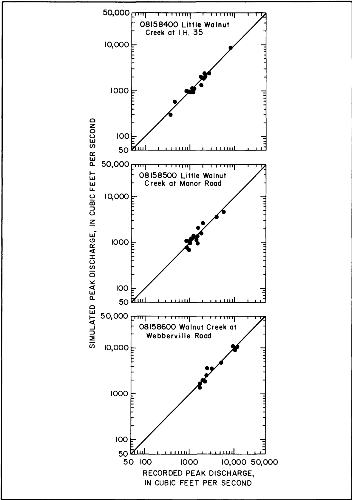
Figure 13.—Recorded and simulated flood-peak discharges from model calibration for streamflow-gaging stations 08158400, 08158500, and 08158600.
