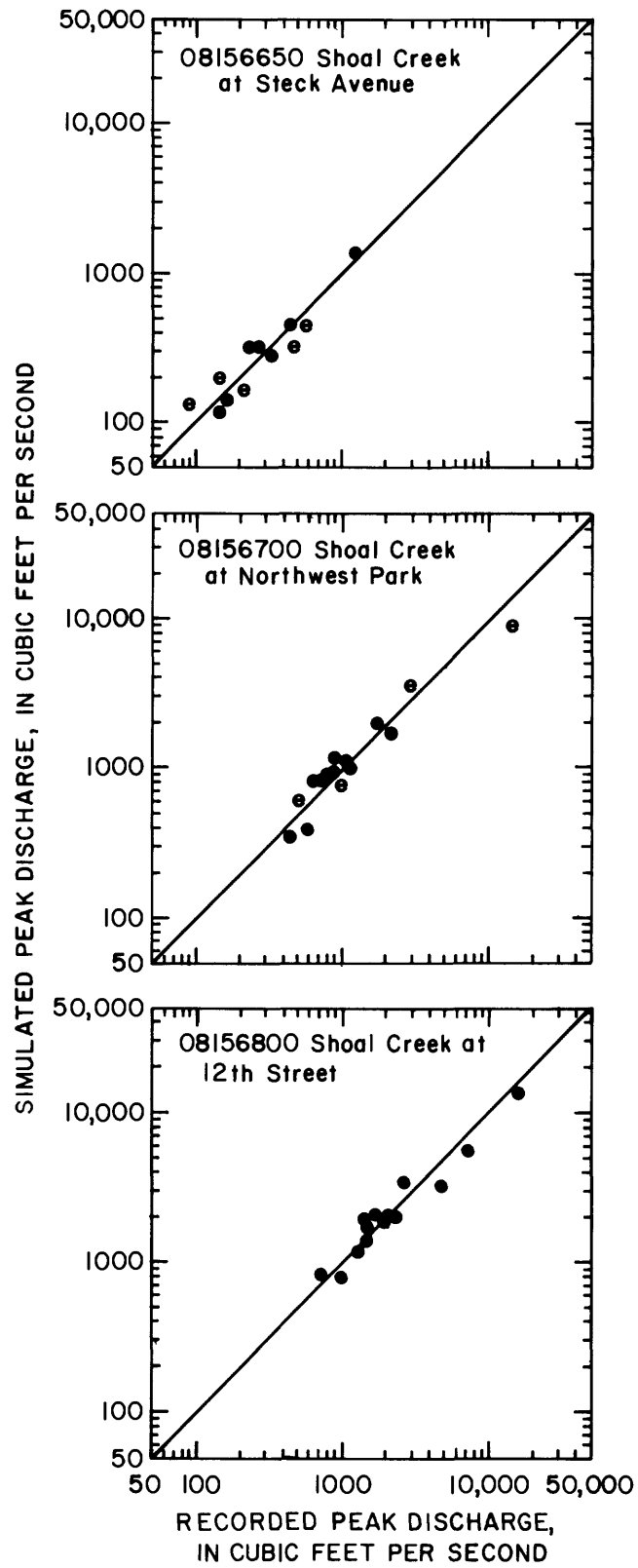
Figure 11.--Recorded and simulated flood-peak discharges from model calibration for streamflow-gaging stations 08156650, 08156700, and 08156800.
