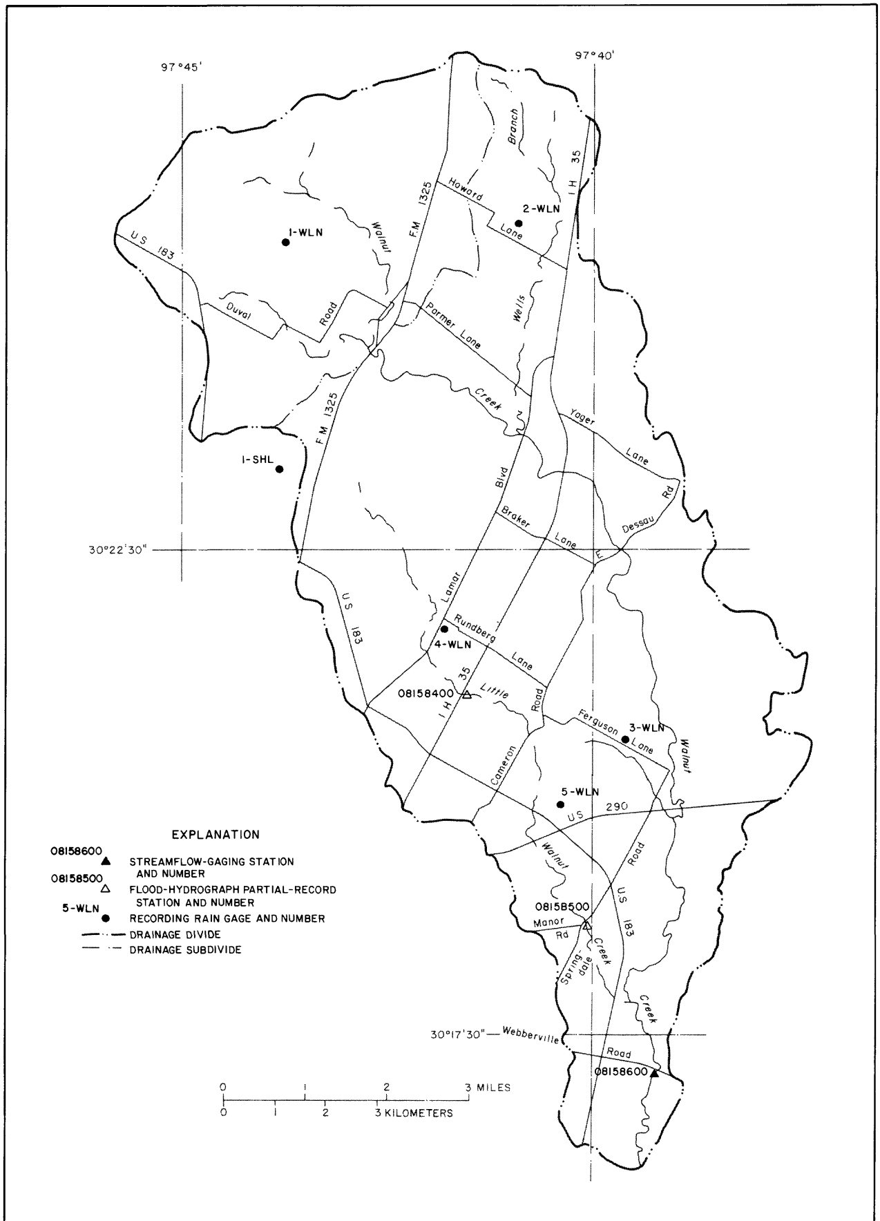
Figure 5.--Walnut Creek and Little Walnut Creek study areas showing location of streamflow stations and recording rain gages.
