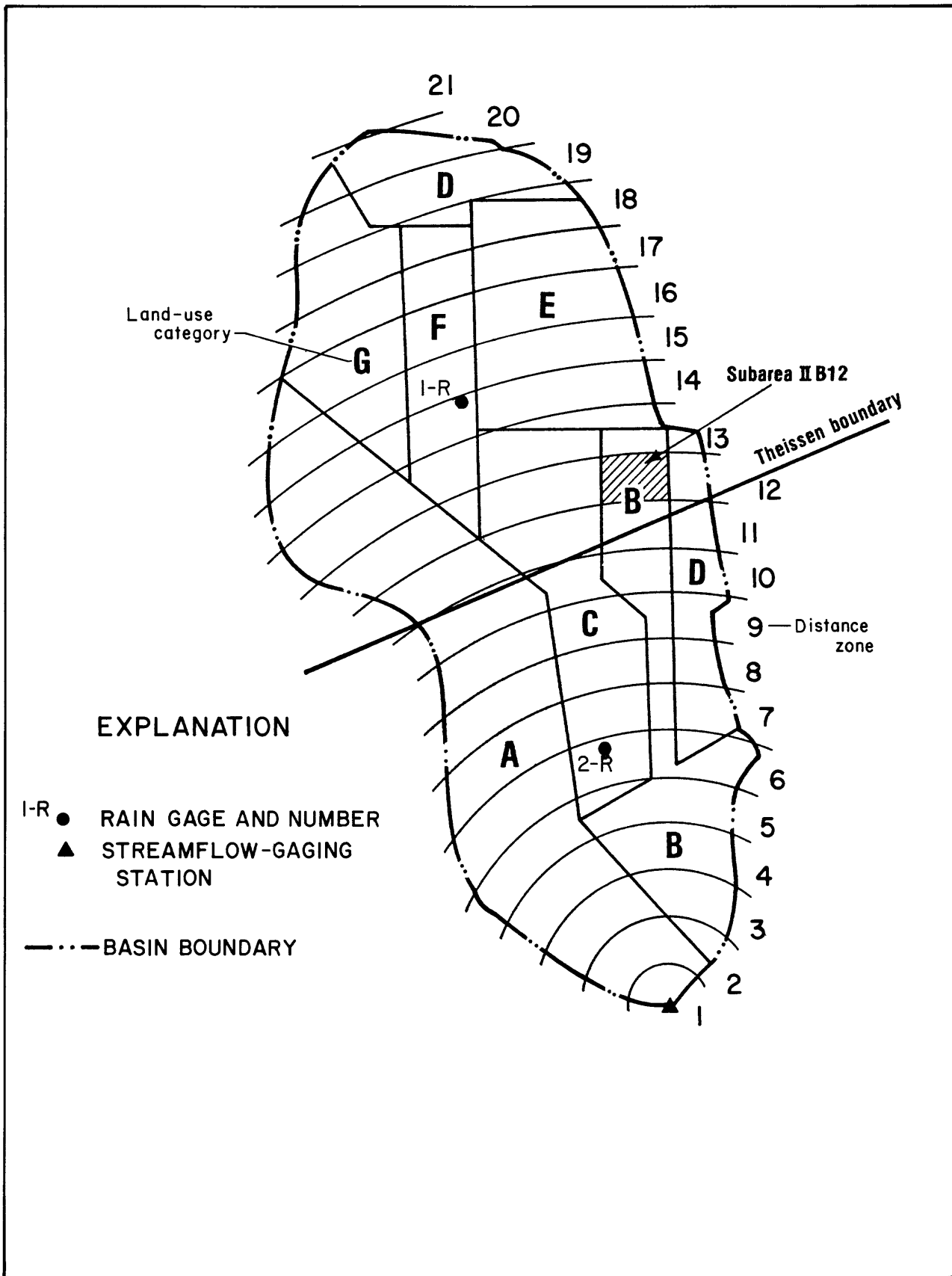
Figure 10.--Sketch showing division of a hypothetical basin into subareas according to location of rain gages, land use, and time of travel.
