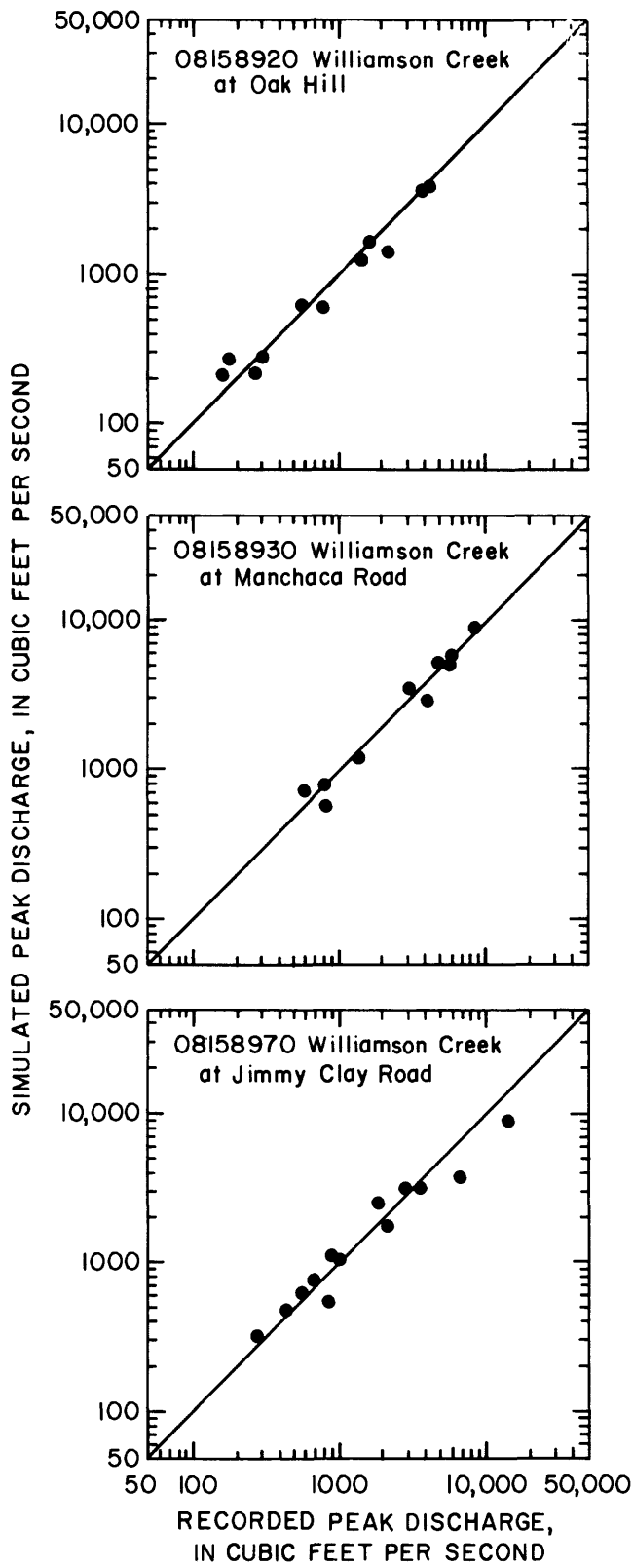
Figure 14.—Recorded and simulated flood-peak discharges from model calibration for streamflow-gaging stations 08158920, 08158930, and 08158970.
