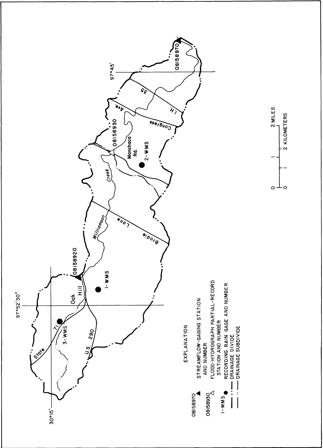
Figure 7.--Williamson Creek study area showing location of streamflow stations and recording rain gages.
