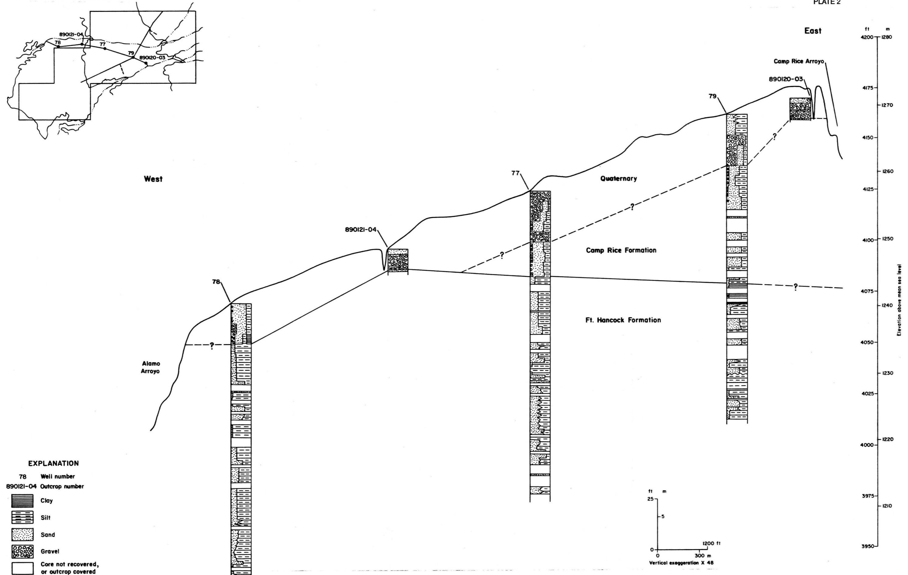
PLATE 2. EAST-WEST STRATIGRAPHIC CROSS SECTION AT THE FORT HANCOCK STUDY AREA, HUDSPETH COUNTY, TEXAS
