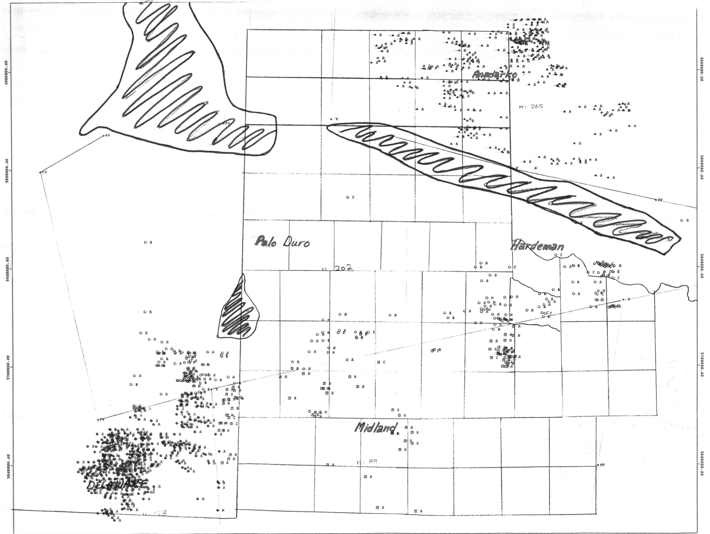
Figure 6. Location of pressure measurements in greater Permian Basin (Delaware, Palo Duro, Hardeman, Midland, and Anadarko Basins) after deletion of data considered unreliable.
