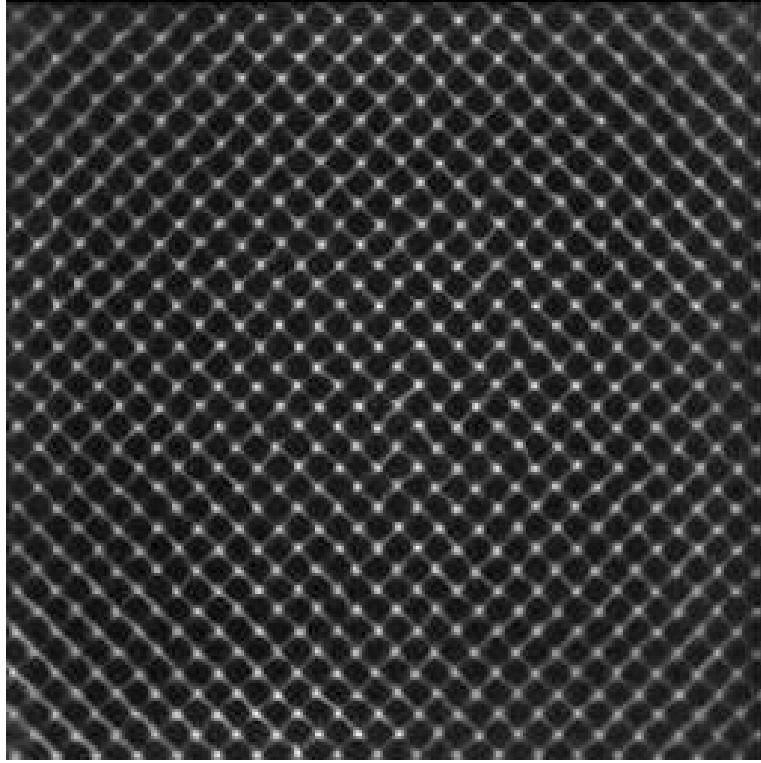
Figure 5.1: A square pattern formed in a square container with four layers of 165\text{ }\mu\text{m} bronze for \Gamma = 3.0 and f_d = 27\text{ Hz} . The pattern is oriented at \pi/4 to the container walls. The region shown is 16 \times 16\text{ cm}^2 .
