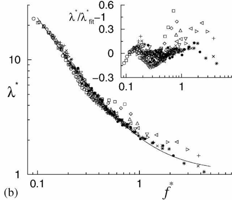
Figure 6.3: Dispersion relation taken for fixed \Gamma at constant particle size and varying particle depth obtained in [180]. The different symbols represent different dimensionless layer depths, N = h/D , where h is the layer depth and D is the grain diameter. The fit is to \lambda^* \equiv \lambda/h = 1.0 + 1.1(f_d/\sqrt{h/g})^{-1.32} . Thus, q_0 = 2\pi/\lambda \sim f_d^{4/3} . The inset show the deviation of the data from the fit.
