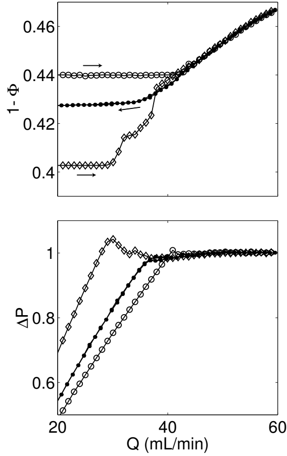
Figure 8.5: Fluidization cycles for increasing flow for two different initial voidages 0.440 ( \circ ), 0.403 ( \diamond ) (a) Voidage vs. flow rate (b) Pressure drop vs. flow rate. Particles are 335\ \mu\text{m} glass spheres with total mass 60 g. The curve with \bullet symbol is for defluidization and is independent of the initial voidage. Protocol: 30 sec ramp between each point with 30 second equilibration time.
