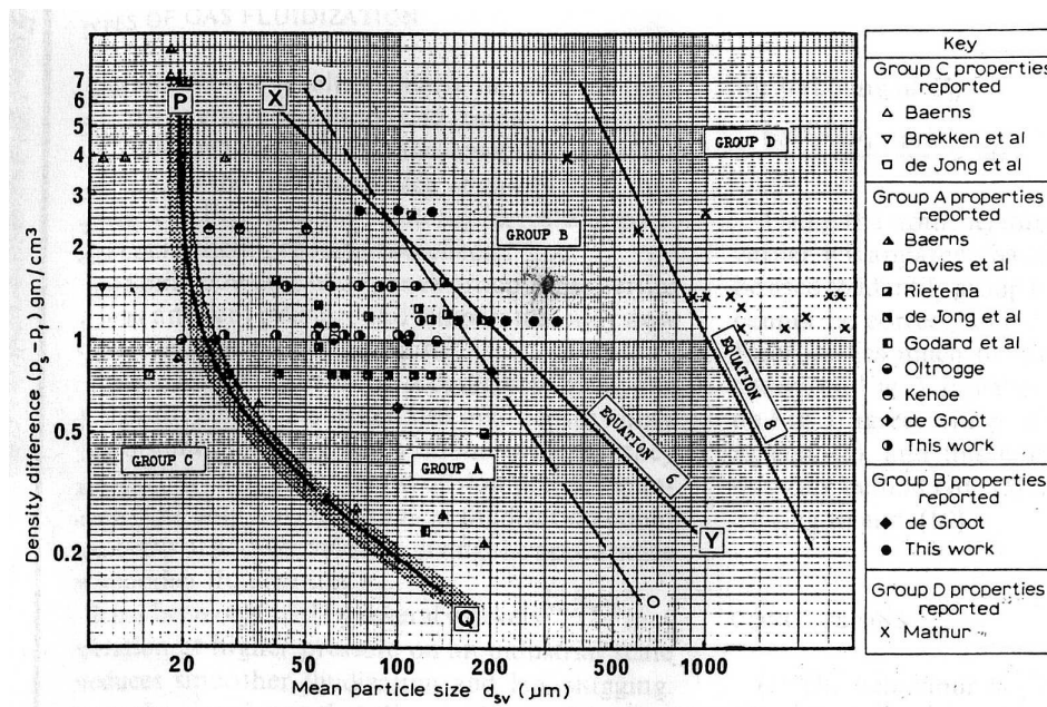
Figure 1.7: The Geldart classification scheme for air fluidized particle.
