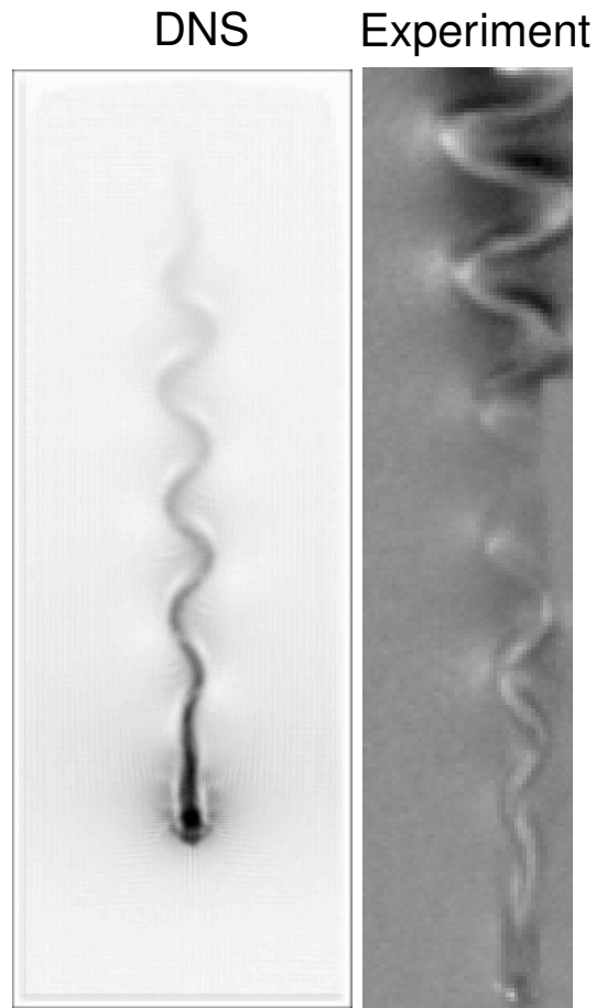
Figure 2.18: Comparison of experiment and DNS results for the sedimentation of a single sphere within a fluid filled gap of 1.1 particle diameters. The agreement is quite good. Courtesy E. Ramos and T.-W. Pan
