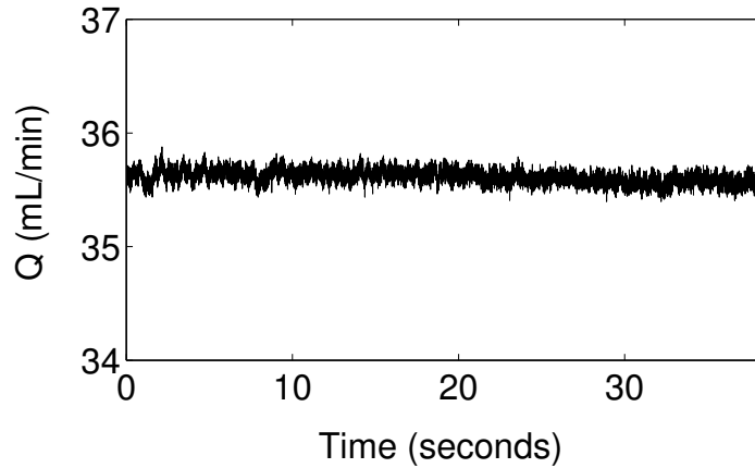
Figure 3.10: The flow measured under control at Q = 35.61 mL/min for 30 seconds. The RMS deviation around the mean is 0.2%.
