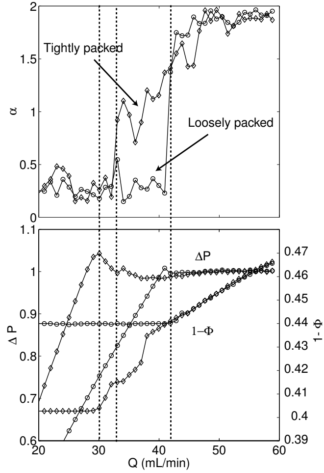
Figure 8.10: Top panel: \alpha as a function of flow rate for fluidization from two different initial packings, tightly packed ( \diamond ) and loosely packed ( \circ ). Note the baseline value of \alpha \approx 0.2 below fluidization. This is due to a slow drift in the system and is discussed in the text. The voidage and pressure data is included for reference in the bottom panel. The dashed lines indicating transitions in bed behavior and protocol for fluidization are the same as those in Figure 8.7.
