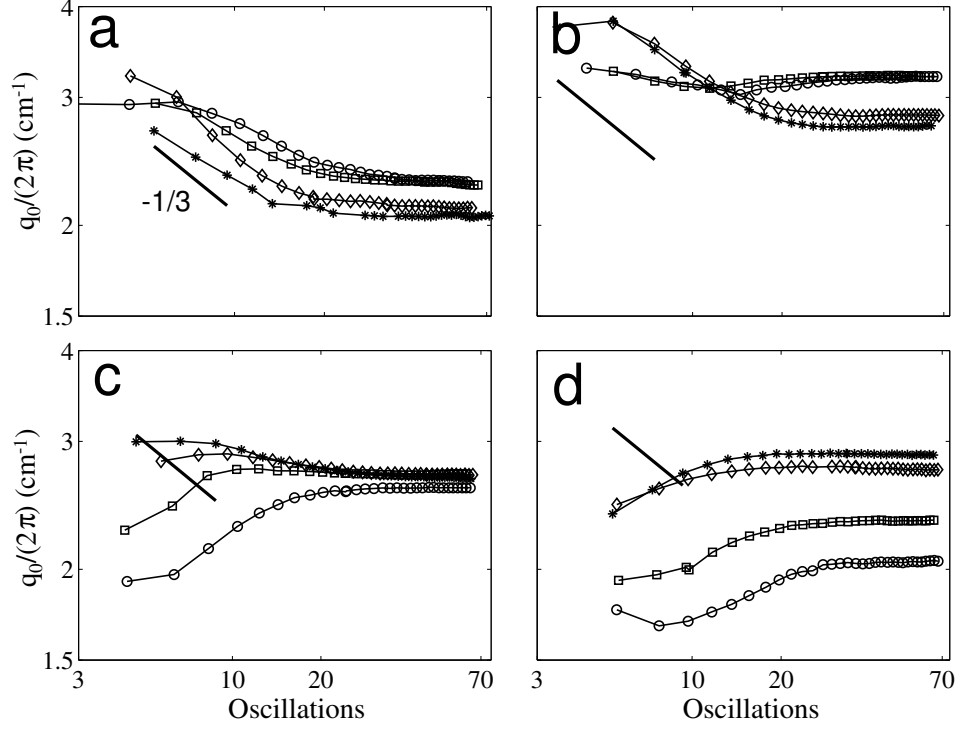
Figure 6.2: The time evolution of q_0 after a rapid jump from initial \Gamma = 2.2 to final \Gamma for constant f_d . In each panel the f_d , N , and initial \tilde{v} of the jumps are (a) 27 Hz, N=4 , \tilde{v} = 3.16 (b) 33 Hz, N=4 , \tilde{v} = 2.59 (c) 40 Hz, N=7 , \tilde{v} = 2.13 (d) 49 Hz, N=7 , \tilde{v} = 1.74 . Each panel shows jumps to increasing final \Gamma and final \tilde{v} denoted by symbols \circ , \square , \diamond , * , with the final \Gamma : (a) (2.65, 2.70, 2.95, 3.18), (b) (2.55, 2.58, 3.10, 3.40), (c) (2.75, 3.20, 3.35, 3.8), (d) (2.48, 2.60, 2.85, 2.98) and the final \tilde{v} : (a) (3.81, 3.88, 4.24, 4.56), (b) (3.0, 3.03, 3.64, 3.99), (c) (2.67, 2.68, 3.10, 3.24), (d) (1.96, 2.06, 2.26, 2.36).
