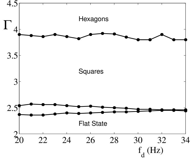
Figure 6.13: Phase diagram for 4 layers showing subcritical behavior at low frequencies. The bifurcation to hexagons for increasing \Gamma is drawn for reference
