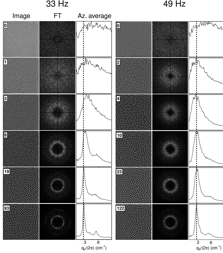
Figure 6.1: The time evolution of pattern after sudden change in control parameters for two different frequencies. For a given frequency, the columns correspond to an image of the granular layer, the modulus of the Fourier transform of the image, and the azimuthal average of the Fourier transform. For (a) 4 layer, f_d = 33 Hz, \Gamma = 2.2 \rightarrow \Gamma = 3.0 , q_0 decreases with time, while in (b) 7 layers, f_d = 49 Hz, \Gamma = 2.2 \rightarrow \Gamma = 3.0 , q_0 increases with time. The dashed vertical lines are to guide the eye and represent the asymptotic value of q_0 . The time units are in plate oscillations.
