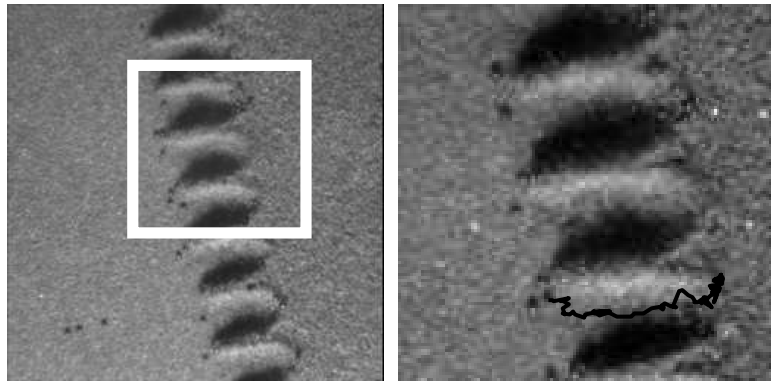
Figure 6.36: Segregation effects in decorated kinks for 650\ \mu m glass spheres into a f_d/2 kink formed in 10 layers of 165\ \mu m bronze spheres shaken at f_d = 40 Hz and \Gamma \approx 4.5 . The large particle remains trapped in the kink but executes a complicated motion along the decoration which leads to transport along the kink.
