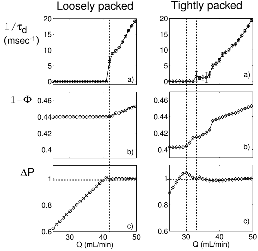
Figure 8.7: Top panels: The decay times of the correlation function, 1/\tau_d , for fluidization from loosely ( \circ ) and tightly ( \diamond ) packed initial conditions. The corresponding pressure and voidage curves are included for reference. Loosely packed: the dashed line denotes where motion begins as indicated by a finite value of 1/\tau_d . The point where the material yields and the point where motion begin are separated by a single flow increment in this experiment. Tightly packed: the leftmost dashed line denotes the value of Q where \Delta P reaches a maximum and 1 - \Phi begins to increase. The dashed line to the right denotes the Q on the tightly packed branch where particle motion begins. Protocol: 30 second ramp with 30 second equilibration time.
