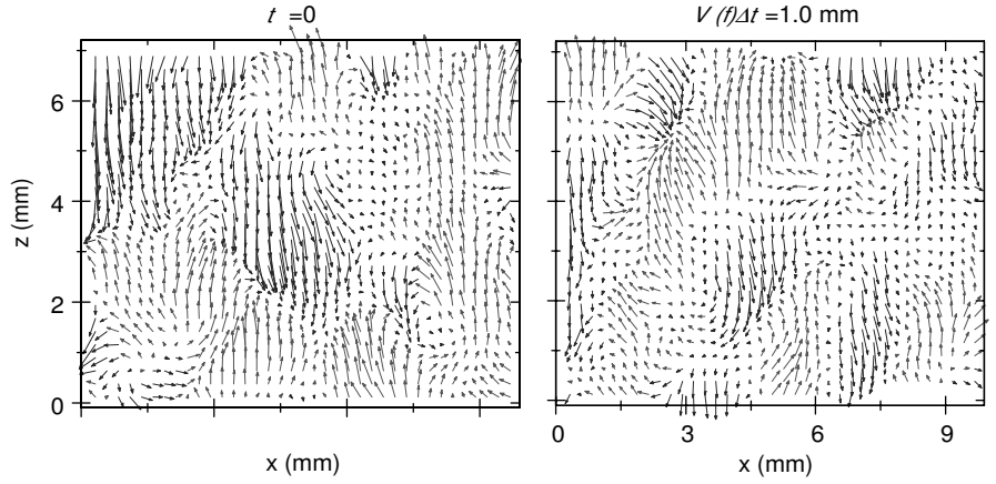
Figure 2.15: The local velocity field showing fluctuating regions in a sedimenting suspension of 50\mu\text{m} particles at Re \approx 10^{-4} , from [164].
