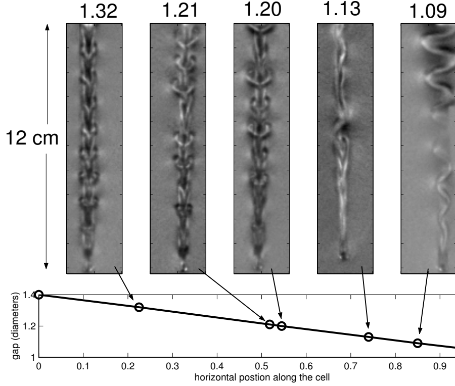
Figure 2.13: The wake behind a 3 mm acrylic sphere falling in water between two plates is a function of the ratio of gap thickness to the ball diameter. In all cases, Re \approx 230 .
