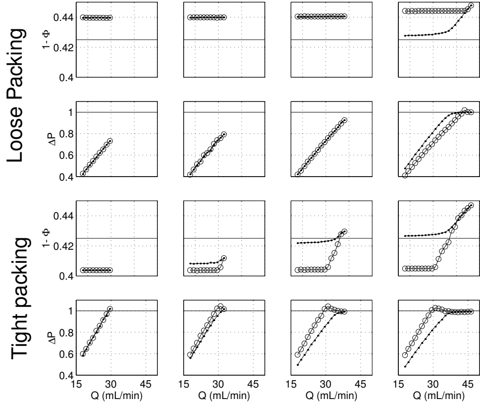
Figure 8.18: Top two rows: voidage and pressure data for fluidization cycles with the same loosely packed initial condition. The panels from left to right show fluidization cycles for increasing turnaround points. Loosely packed initial condition. Bottom two rows: same as the top two rows, but for a tightly packed initial condition. Increasing flow denoted as \circ , while decreasing flow as \bullet . If the yield stress is not broken, the paths are reversible for slow changes in Q . Once the material has yielded, defluidization follows a different path. The solid black lines in the voidage plots indicate the voidage obtained for slow defluidization from above RLP. The solid black line in the pressure plot denotes \Delta P = 1 .
