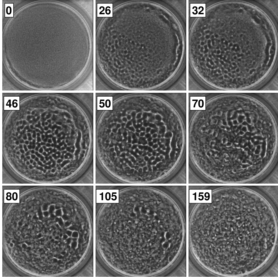
Figure 6.30: Transient growth and decay of square patterns oscillating at f/6 . At t = 0 , \Gamma is increased from 2.2 to 9.2 at f_d = 83Hz , N = 15 .
