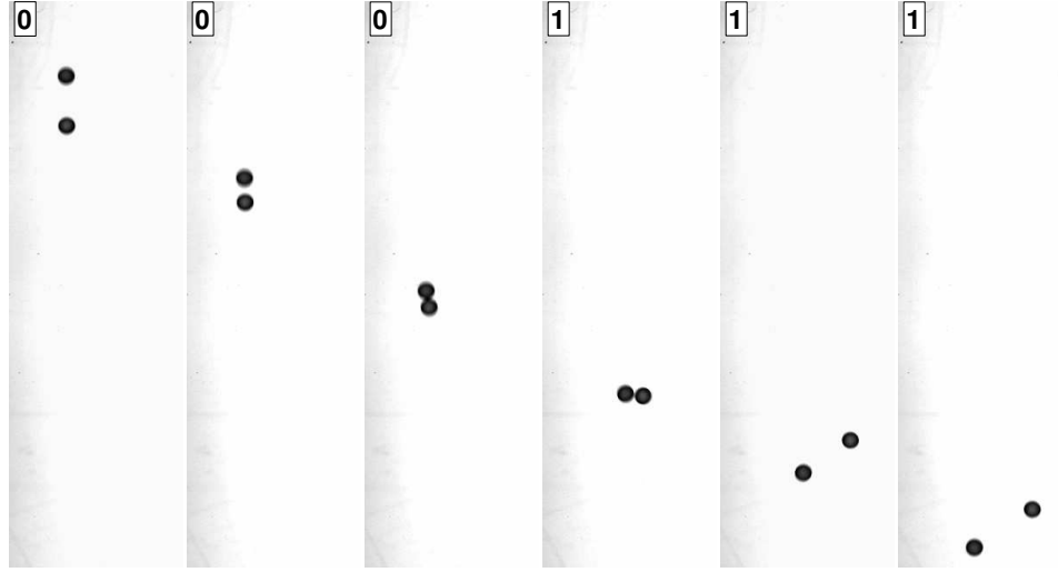
Figure 2.14: Two particles falling in water draft, kiss, and tumble as they fall. Images courtesy of Eduardo Ramos.
