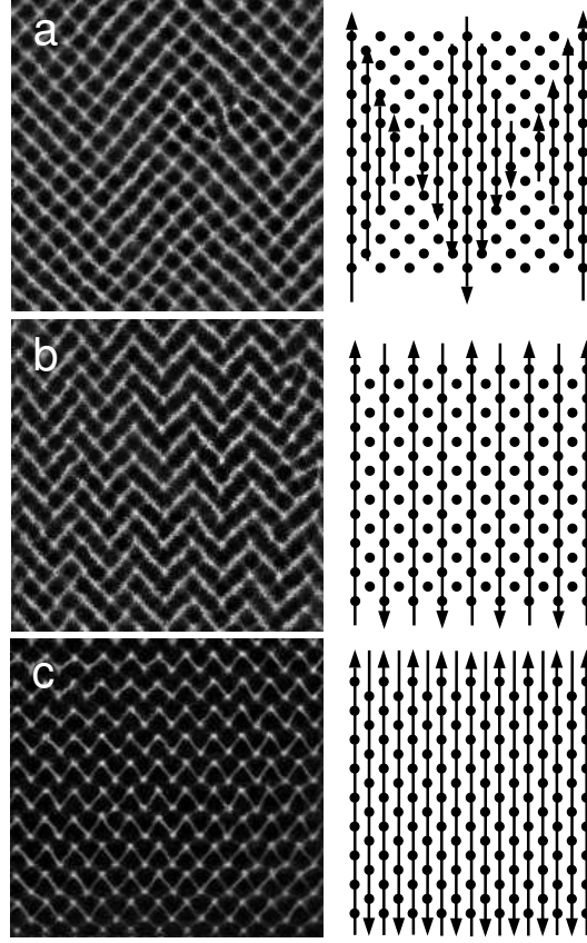
Figure 5.12: (a) and (b) are images taken at f_d=32 Hz and \Gamma = 2.9 under frequency modulation for constant f_{ms} = 4.0 Hz and increasing f_{mr} , where (a) f_{mr} = 1 Hz, (b) f_{mr} = 2.25 Hz. The wavenumber of the mode increases with increasing f_{mr} . To the right of each picture, a schematic shows the relative motion of the rows of the crystal in the given mode. The mode shown in (c) is never excited over the range of f_{ms} and is an image of the lattice in resonance peak I, with \Gamma = 2.65 and f_d = 21 Hz.
