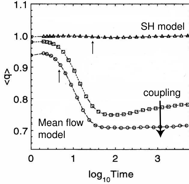
Figure 6.12: The behavior of the wavevector for a numerically integrated Swift-Hohenberg model ( \triangle ). \square and \circ are for a pattern formation model which couples the rolls to a mean flow. The evolution changes as the coupling changes. Taken from [37].
