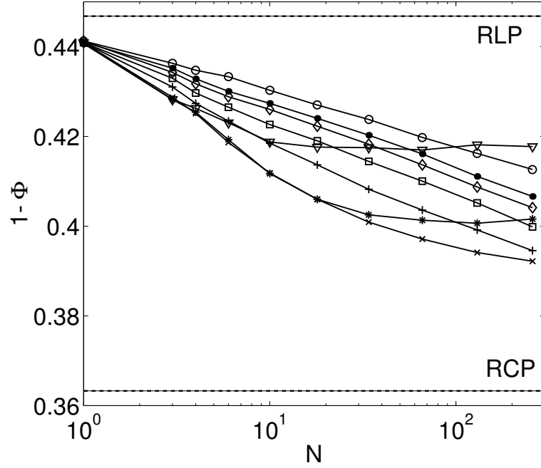
Figure 8.2: The voidage of the bed decreases as the number of toggles increases. Here duty cycle is fixed to 1/3 on 2/3 off and the entire cycle lasts 2 seconds. Q_{\max} has values of (\circ, \bullet, \diamond, \square, +, \times, *, \nabla) , (0, 17.3, 27.2, 48.6, 71.3, 94.1, 116.2, 136.5) mL/min.
