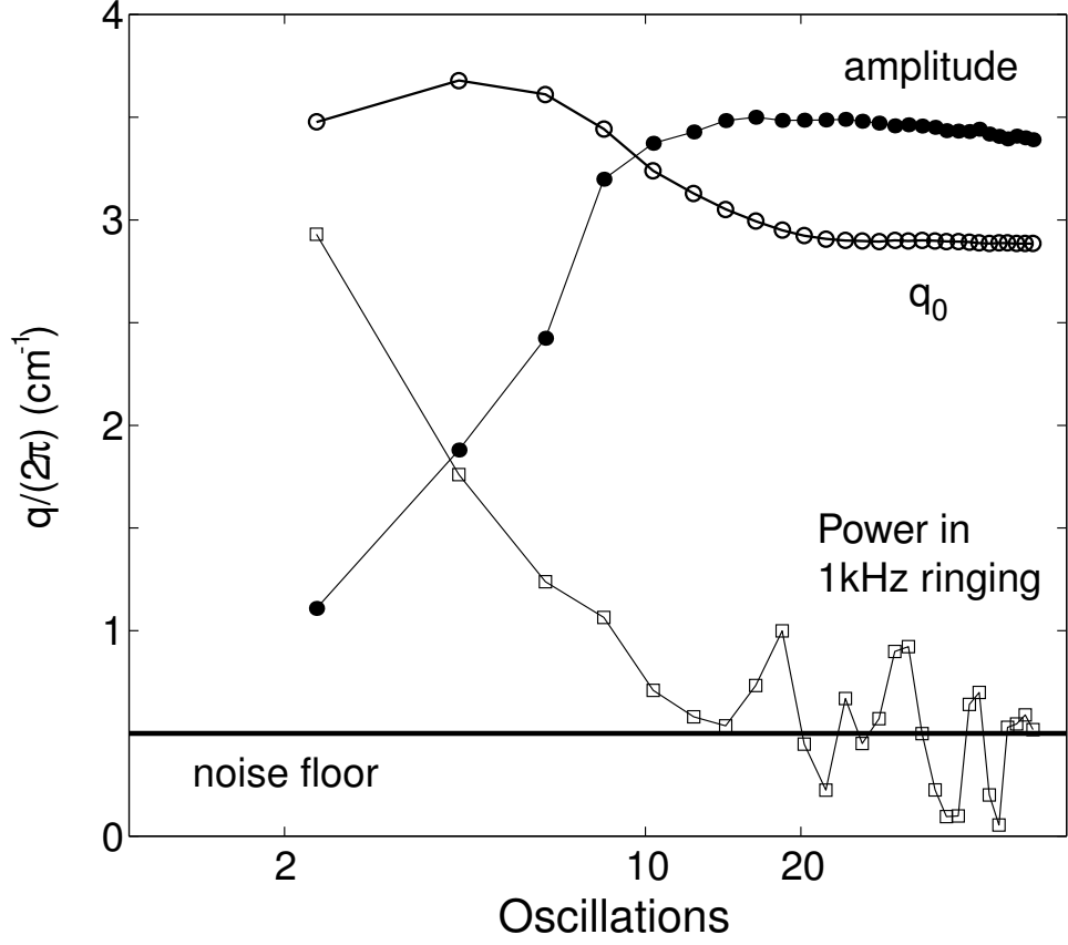
Figure 6.10: The changes in different layer characteristics during the jump to \tilde{v} = 3.5 at 33 Hz. q_0 (○) decreases until the layer is fully fluidized as measured by the integrated power in the 1 kHz ringing mode (□). A measure of the amplitude (●) of the pattern increases and reaches a peak before the layer is fully fluidized.
