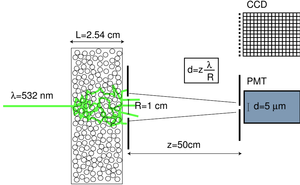
Figure 3.12: The scattered light in the experiment is detected by either a PMT or a CCD camera. The pinhole in front of the PMT images one coherence area, whereas each element of the CCD, 10 \times 10 \mu\text{m} , images slightly less than one coherence area. A side-view of the CCD is shown.
