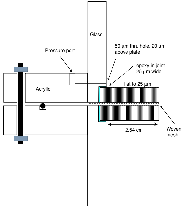
Figure 3.9: Schematic of a proposed fluidized bed using a porous glass plate to sandwich mesh. Different meshes would be used to vary pressure drop across the distributor.
