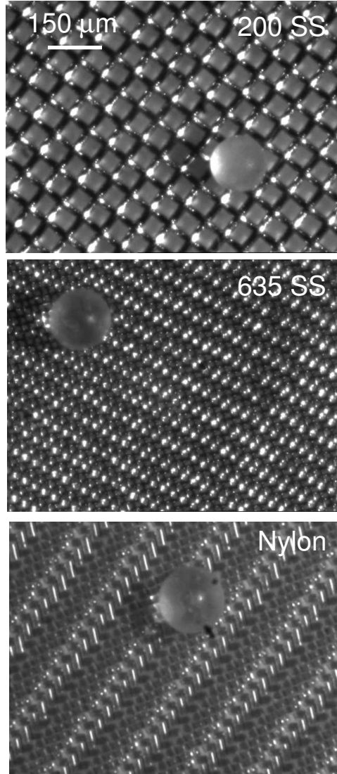
Figure 3.6: Different meshes used as flow distribution elements. A combination of stainless steel and nylon mesh produces a uniform flow distributor. A 100\ \mu\text{m} glass sphere is shown for scale reference.
