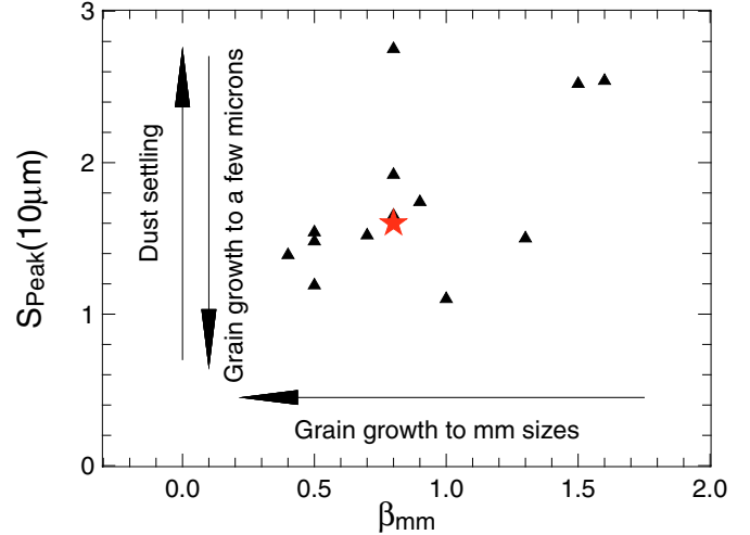
Fig. 13. Strength of the 10\mu\text{m} silicate features as a function of the millimetre opacity slope for the T Tauri stars listed in Table 6. IM Lupi is represented by the red star. The effect of grain growth and dust settling are schematised by arrows.
