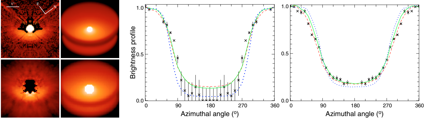
Fig. 8. Scattered light images of the best models compared to observations. Left panel: the upper row corresponds to the images at 0.606\,\mu\text{m} and the lower row to those at 1.6\,\mu\text{m} . Synthetic maps ( right ) were convolved by the core of the PSF (up to 5 pixels from the peak). Central panel: 0.6\,\mu\text{m} azimuthal brightness profile. Right panel: 1.6\,\mu\text{m} azimuthal brightness profile. In both central and right panels , the red dashed line correspond to the best fit of the scattered light only, the full green line to the best fit of all observations simultaneously and the blue dotted to the scattered light images with porous grains. The azimuthal angle is 0^\circ in the front side of the disc, i.e. towards bottom in the first panel.
