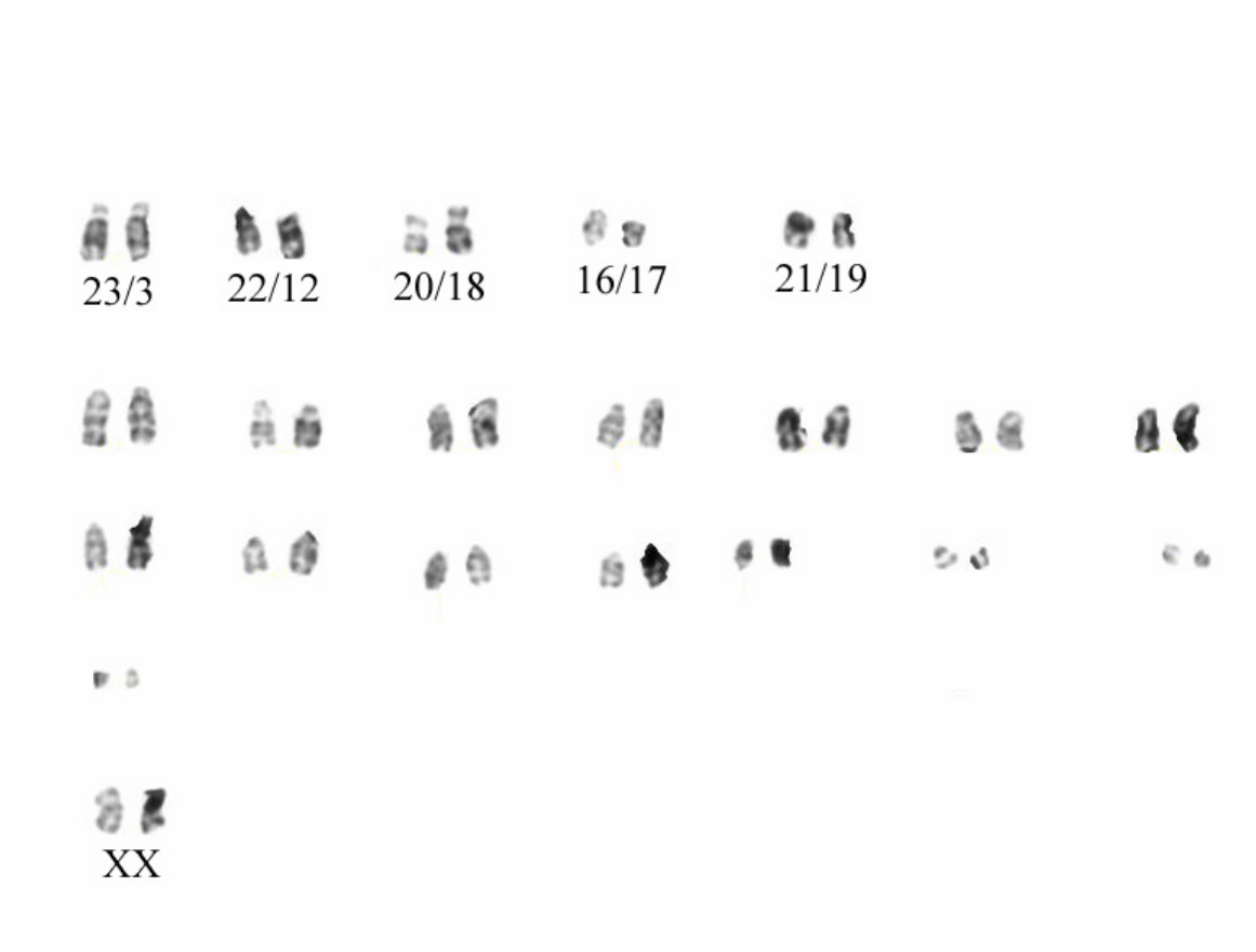
Figure 2.2. Karyotype of R. velilla from Ecuador ( 2n = 42 ). Numbers below biarmed chromosomes represent arms involved in the centric fusions of those chromosomes (chromosomal nomenclature following Bickham 1979a and 1979b).
