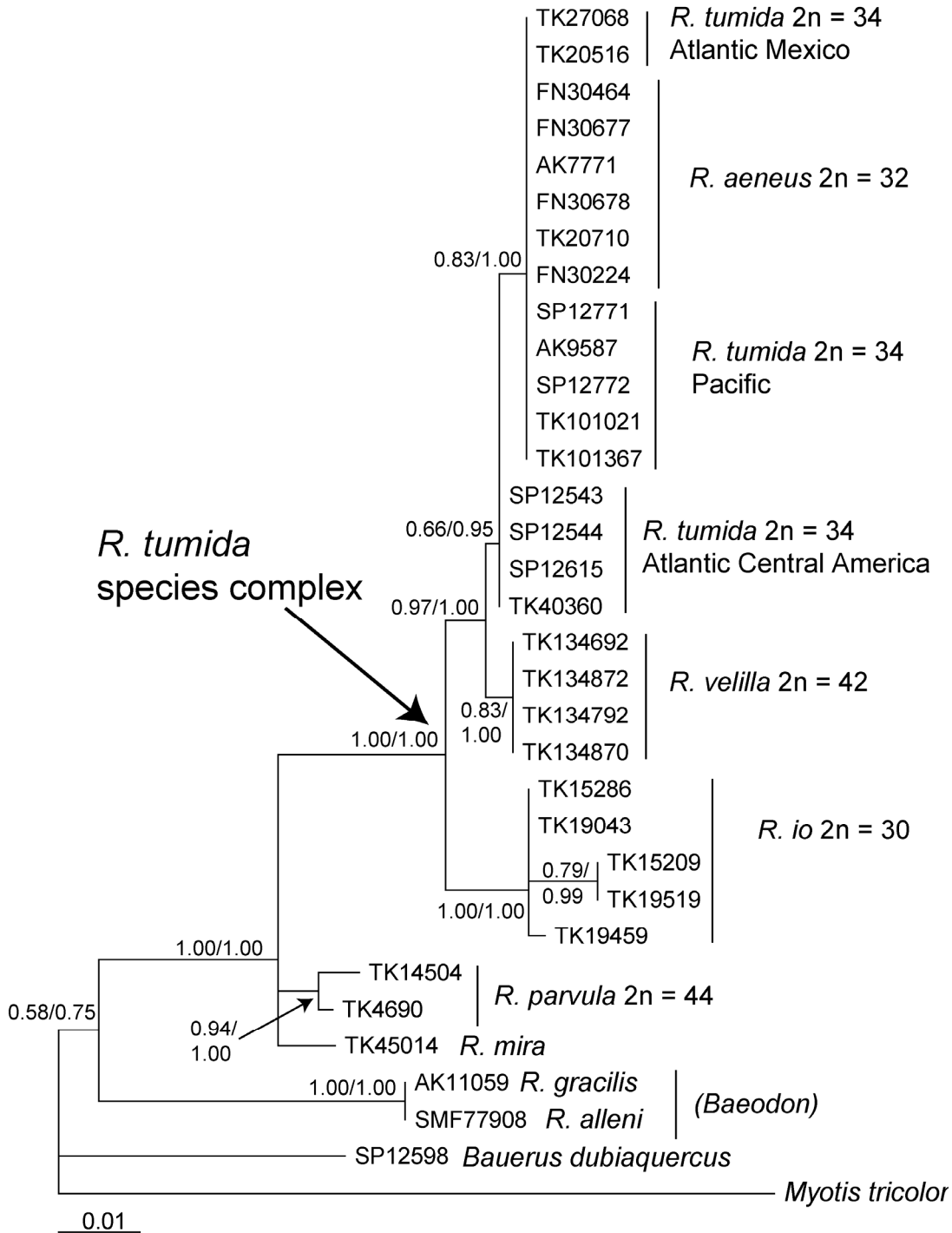
Figure 3.3. Maximum likelihood phylogeny of Rhogeessa based on ZFY sequences. Numbers at nodes represent ML bootstrap proportions followed by Bayesian posterior probabilities. Sample names correspond to those found in Appendix A.
