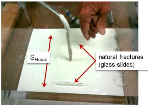
Figure 4. A test block in preparation with two glass slides set in the middle layer of plaster as it is being poured.
