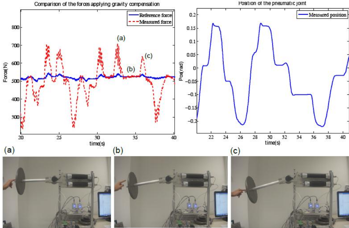
Figure 12: Gravity Compensation: A torque is commanded to compensate for the weight of a heavy load of 12[kg] for a varying position. This situation is similar to holding a leg in the air with low gains. In (a), (b) and (c) we show the sequence of movements of the heavy load upon small contact interactions with a user. Notice that the spikes correspond to the external pushes.
