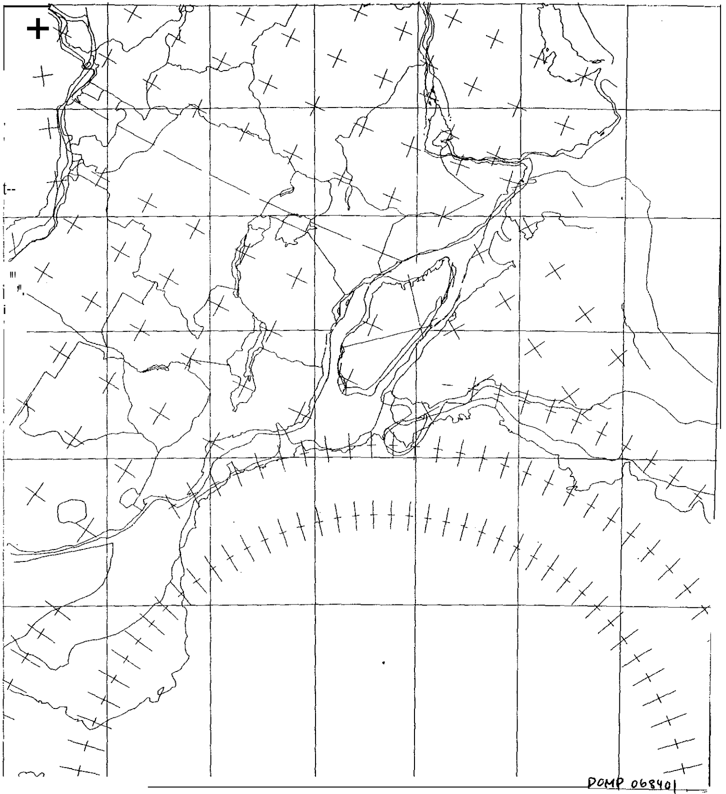
Figure 2. Gondwana Reassembly (Lawver et al., 1984)
