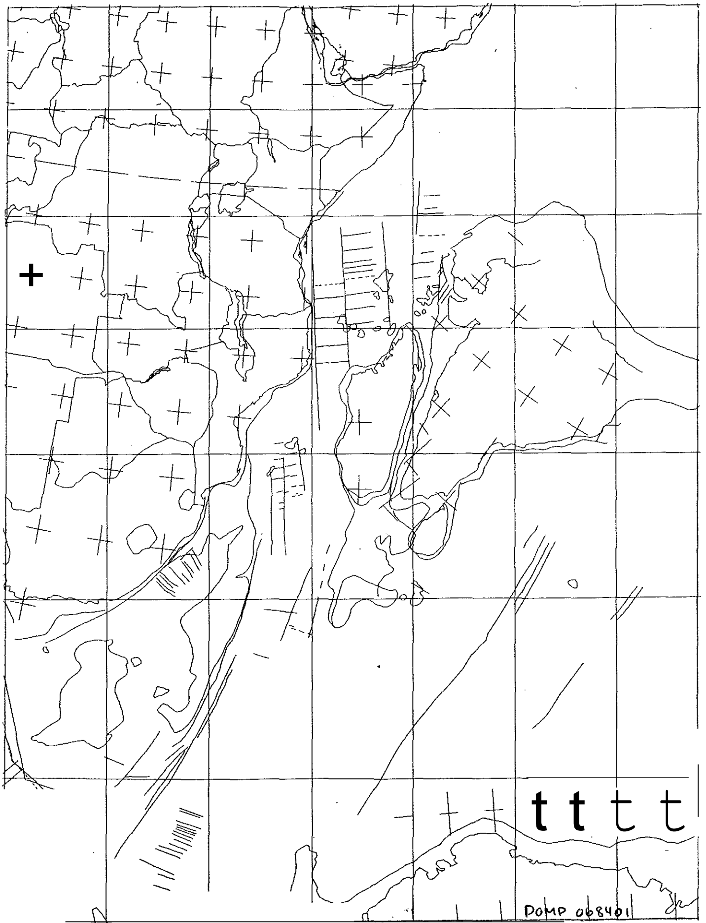
Figure 4. Recon unction at Anomaly 34 Time.
