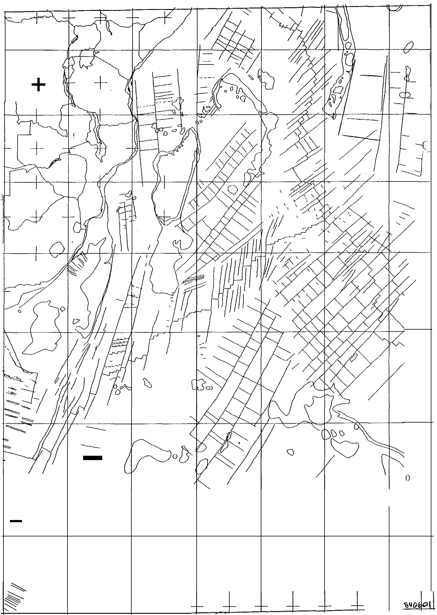
Figure 8. Linear Magnetic Anomaly and Tectonic Features Data Base.
