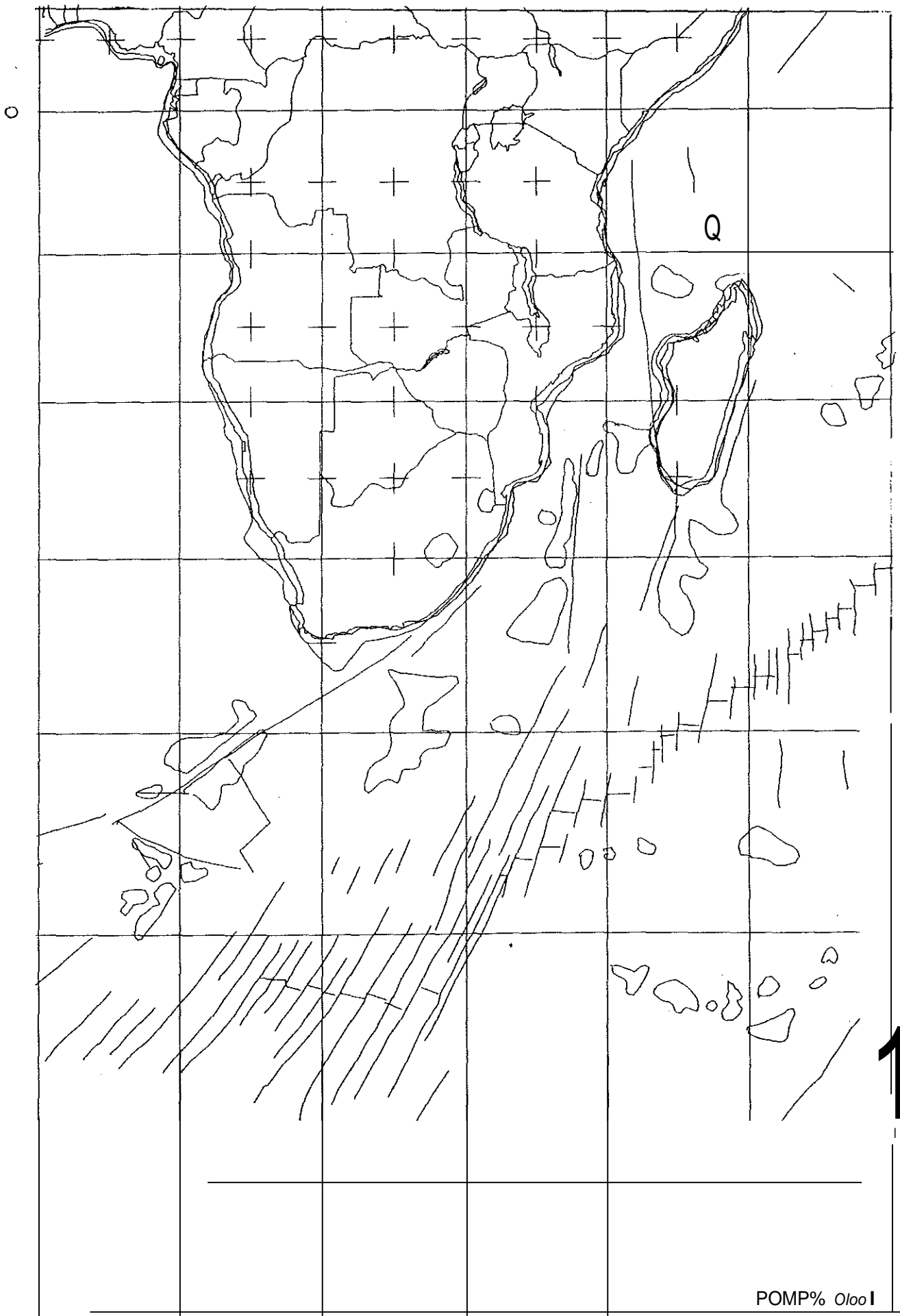
Figure 9. Tectonic Lineations from Haxby (1984).
