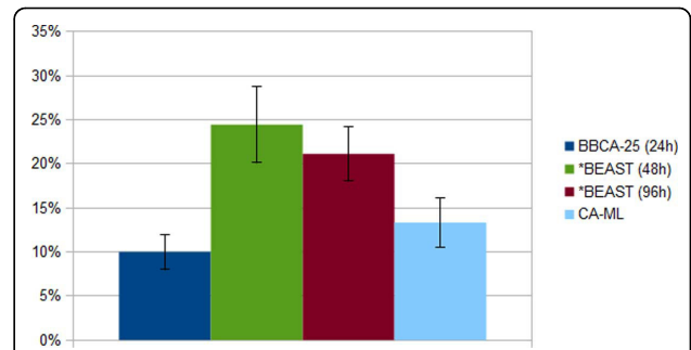
Figure 5 Average species tree estimation error (and standard error bars) on the ten Laurasiatheria 500 bp simulated datasets using BBCA, *BEAST and concatenation; BBCA is run with a 24-hour time limit on each 25-gene bin, and *BEAST is run with a 48-hour or 96-hour time limit.
