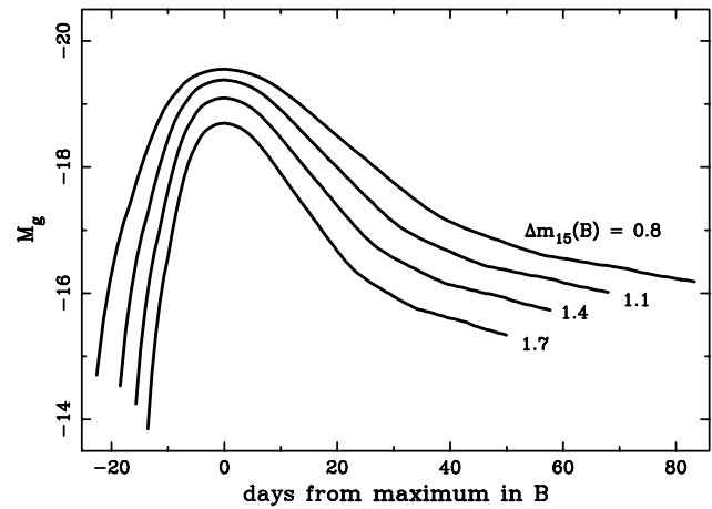
Figure 12. Sample SN Ia rest-frame g -band light curves for four values of \Delta m_{15}(B) = 0.8, 1.1, 1.4, and 1.7 .
