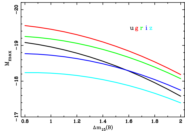
Figure 13. Resulting peak absolute magnitudes for a SN Ia at zero redshift in the SDSS ugriz system as functions of \Delta m_{15}(B) . The curves are analogous to those shown in Figure 8 of Phillips et al. (1999).
