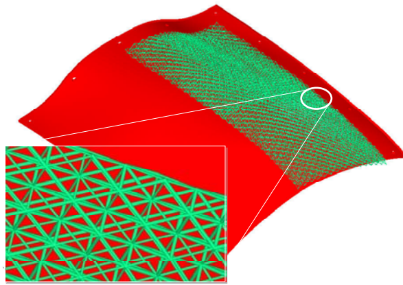
Fig 10 Cover plate with optimized lattice structure (shown on only half of the plate).
