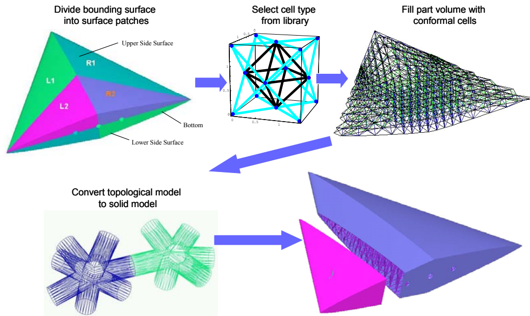
Fig. 6 Cellular modeling approach.
