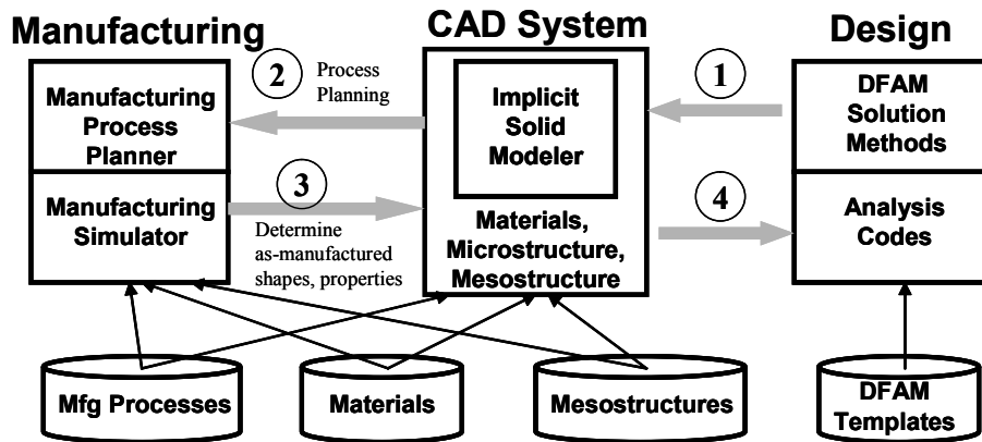
Fig. 5: DFAM System and Overall Method.
