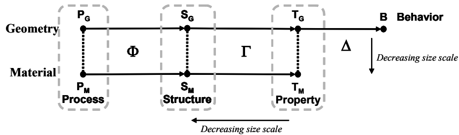
Fig. 3: Expanded DFAM Framework with Geometry and Material Layers.
