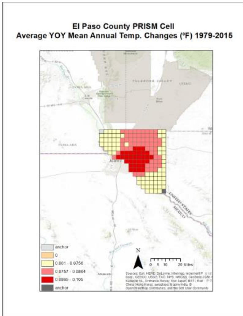
Figure 19 – Average YOY mean annual temperature changes in El Paso County from 1979-2015
