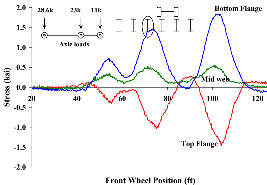
Figure 5.30 Goliad test results for longitudinal stringer S3
