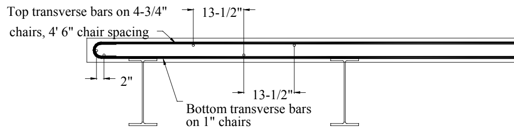
Figure 6.9 Longitudinal reinforcement
