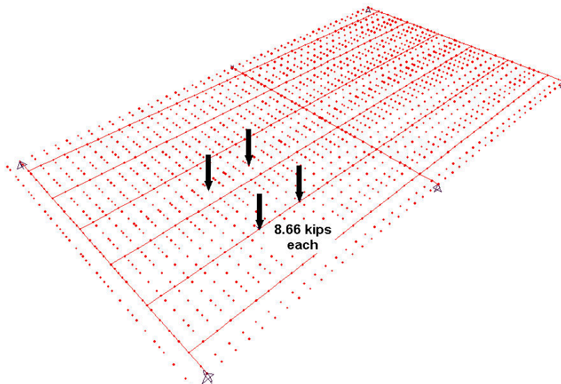
Figure 4.29 Loading for field test in stringer 2
