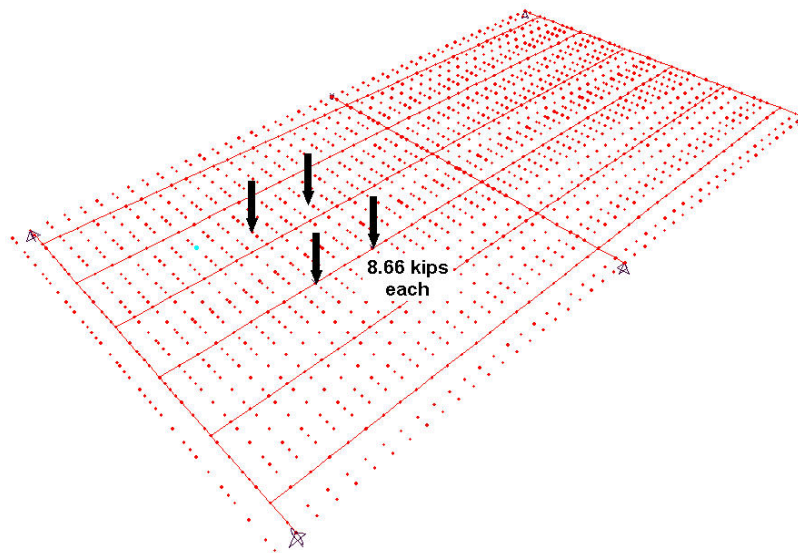
Figure 4.30 Loading for field test in stringer 3
