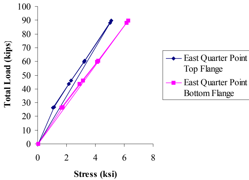
Figure 6.38 Stringer S3: load vs. top and bottom quarter point flange stresses
