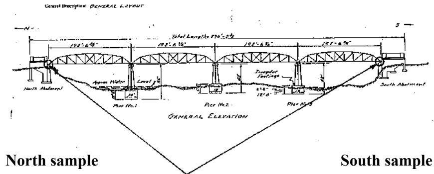
Figure 2.13 Steel sampling locations
