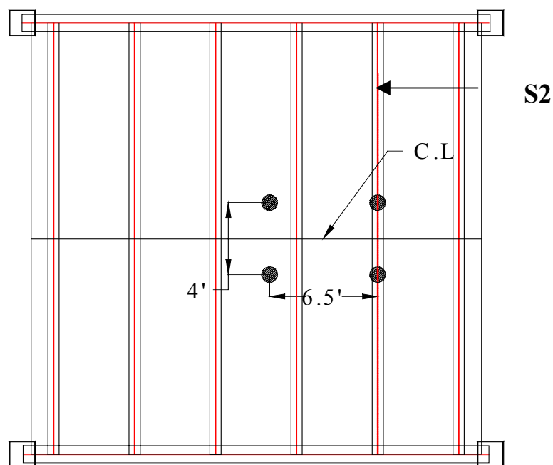
Figure 6.20 Load position for centerline testing of stringer S2
