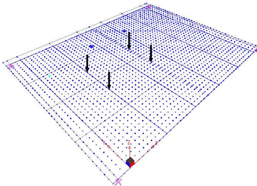
Figure 6.24 Point load position for longitudinal stringer S2 loading
