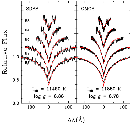
FIG. 3.— Model fits (red lines) to the Balmer line profiles of J1529+2928 from the SDSS (left panel) and Gemini (right panel) spectroscopy. Both fits show that H \gamma and H \beta are slightly filled in due to the flux contribution from a relatively cool starspot.
