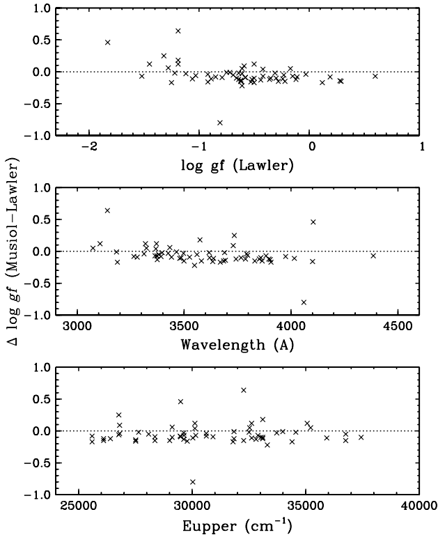
FIG. 4.—Comparison of experimental transition probabilities from Musiol & Labuz (1983) to our transition probabilities as function of our transition probability or \log(gf) , wavelength, and upper level energy.
