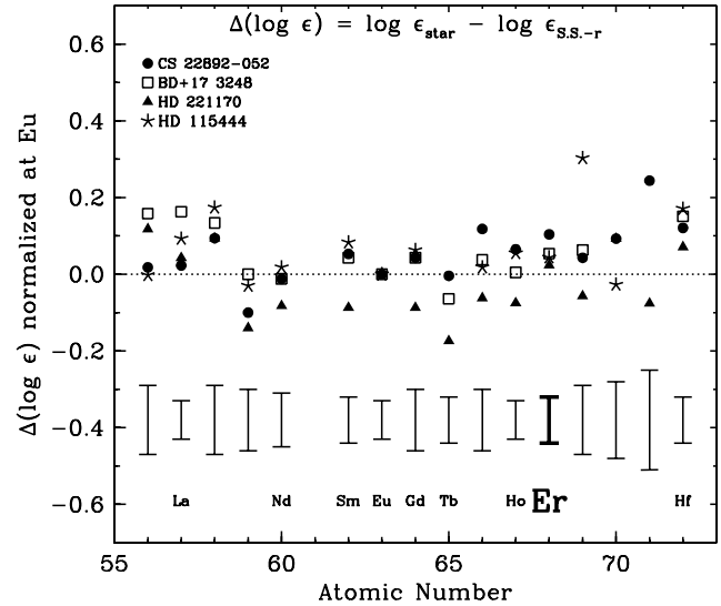
FIG. 10.—Comparison of rare-earth abundances in four r -process-rich stars to the solar-system r -process-only abundances. The solar-system values are taken from Simmerer et al. (2004). The stars, identified in the figure legend, are those that have been analyzed in this series of papers. For each star, the abundance differences have been normalized such that \Delta(\log \epsilon(\text{Eu})) = 0 . The dotted line indicates equality between the stellar and solar-system r -only abundances. The error bars are the means of the sigma values of individual stellar abundances. The abundances for the named elements are taken from the present and earlier papers of this series, and other abundances are taken from the original stellar analyses of the stars.
