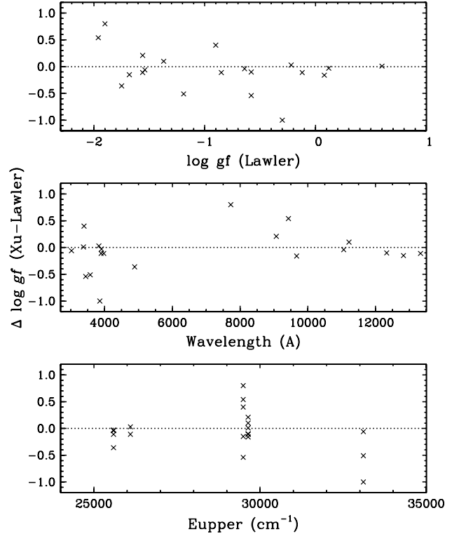
FIG. 5.—Comparison of theoretical transition probabilities from Xu et al. (2003) to our transition probabilities as function of our transition probability or \log(gf) , wavelength, and upper level energy.
