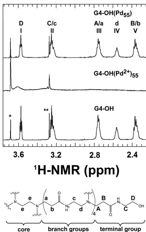
Fig. 6 (Top) ^1\text{H} NMR spectra of G4-OH, G4-OH( \text{Pd}_{55} ), and G4-OH( \text{Pd}_{55} ). The peak marked with a single asterisk arises from the dioxane internal standard, and the peak marked with a double asterisk arises from residual methanol. (Bottom) Schematic representation of G4-OH indicating the lettering scheme used to identify the methylene and nitrogen groups. Reprinted with permission from ref. 20. Copyright 2009 American Chemical Society.
