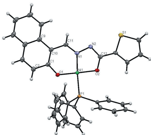
Fig. 2 The molecular structure of complex 5 , with displacement ellipsoids drawn at the 50% probability level.
